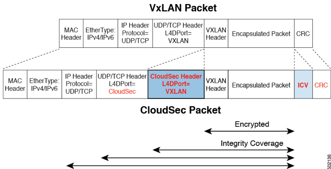
Figure 2: CloudSec Packet
