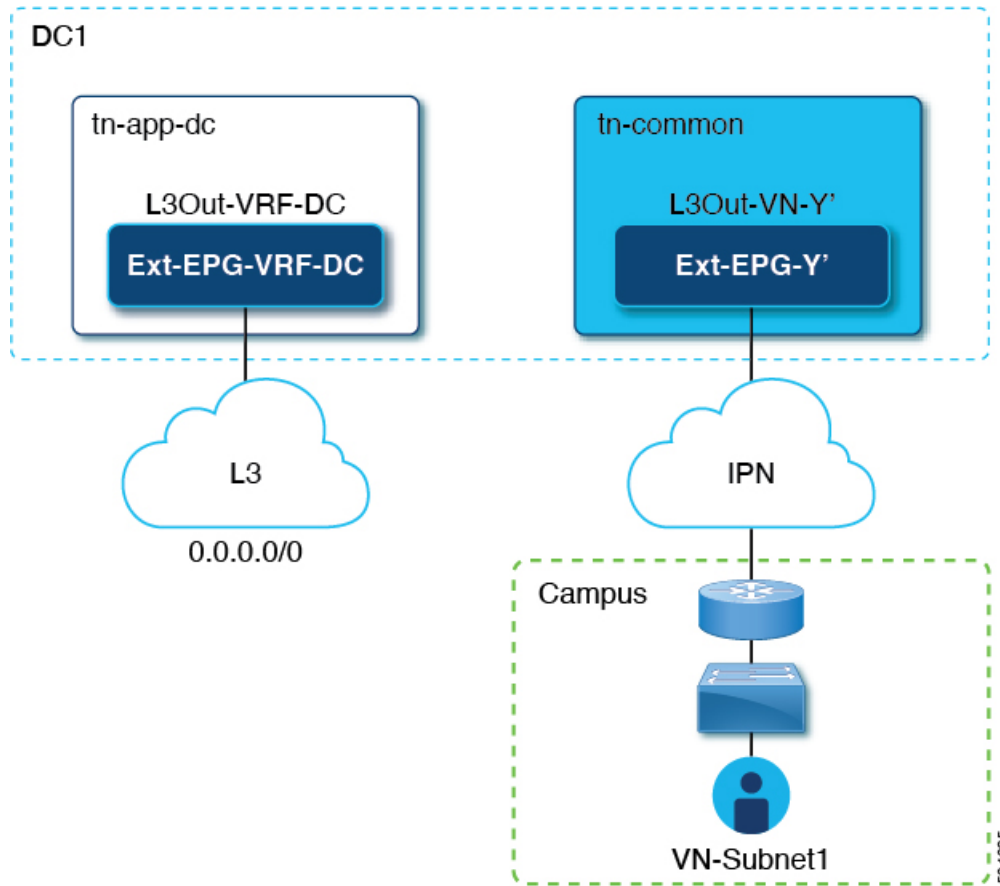
Figure 27: L3Out connection
