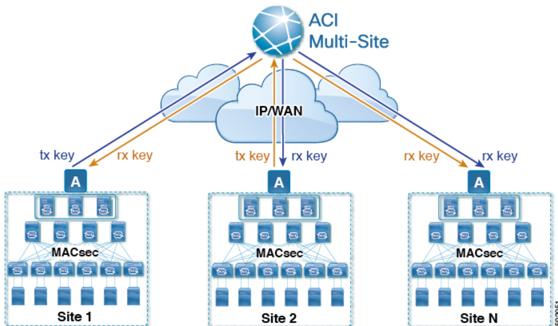
Figure 13: CloudSec Key Distribution
