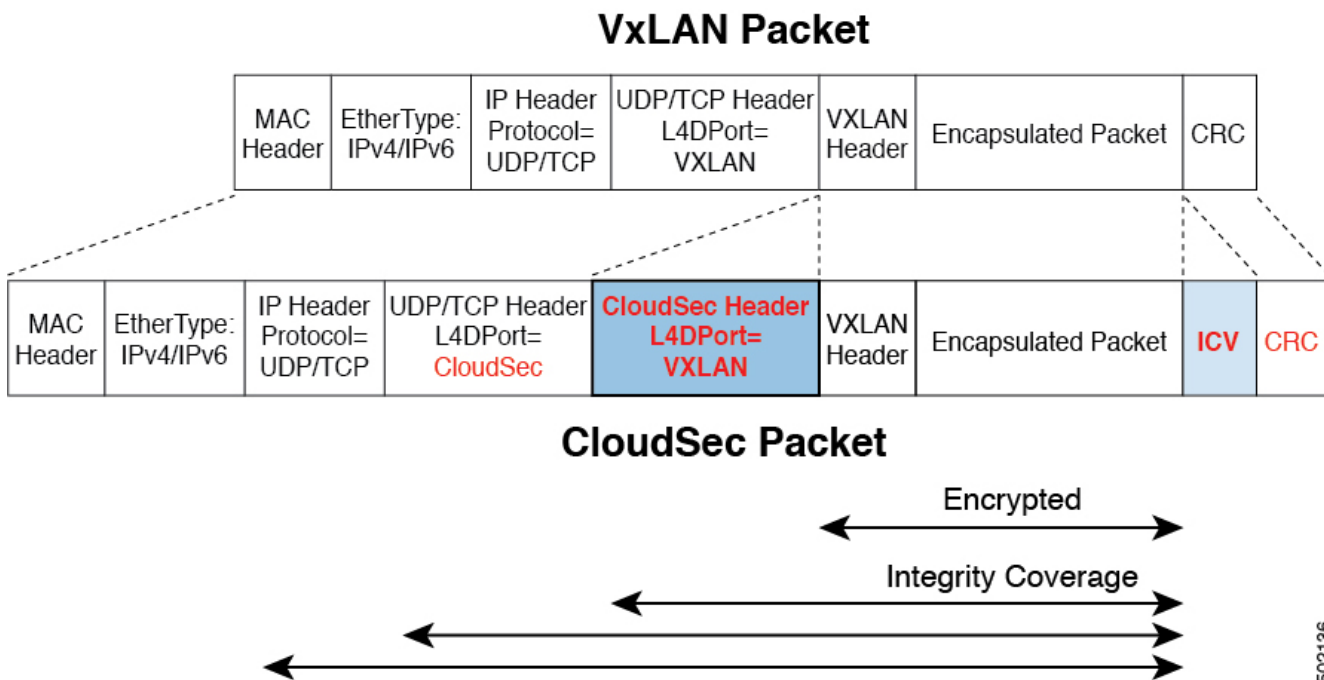
Figure 2. CloudSec Packet
