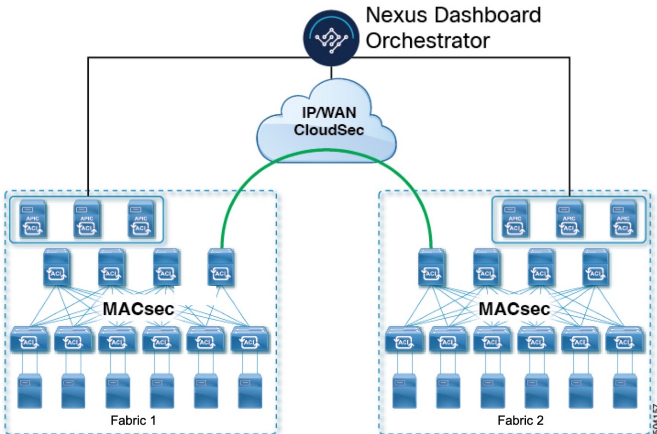
Figure 1. CloudSec Encryption
