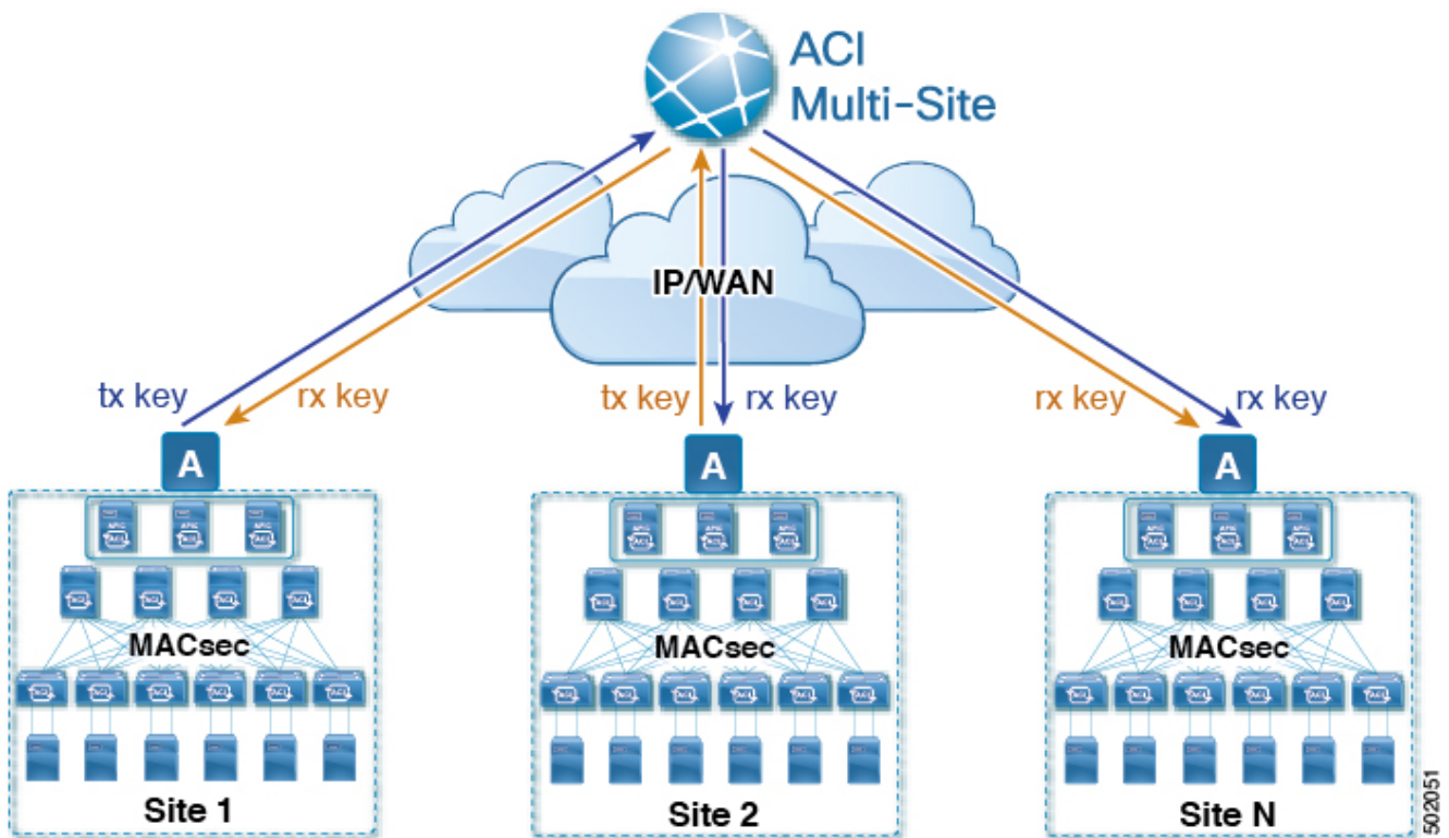
Figure 3. CloudSec Key Distribution
