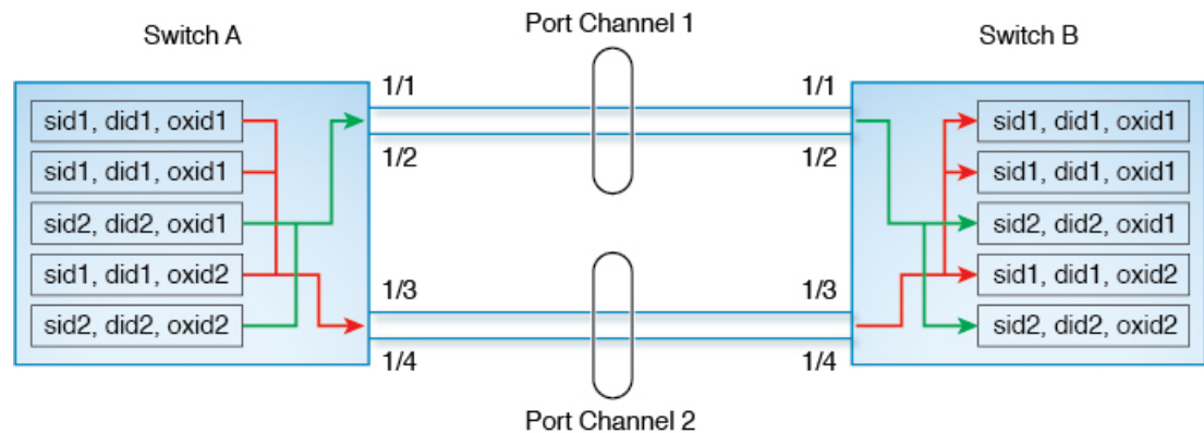
Figure 48: Flow Based Load Balancing
