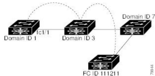
Figure 47: Fibre Channel Routes
