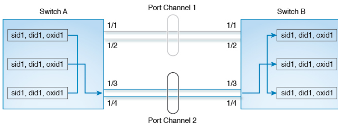
Figure 50: ECMP Hashing Method
