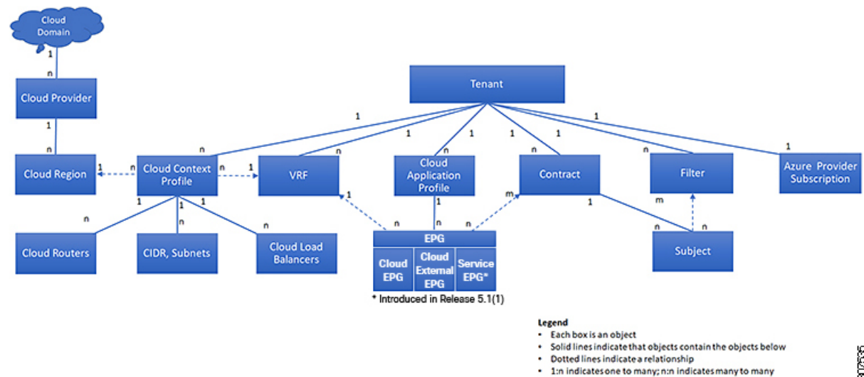
Figure 13: Tenants
