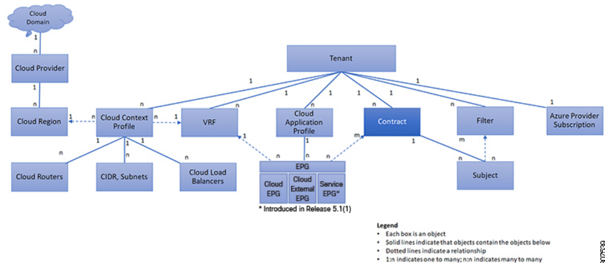
Figure 17: Contracts
