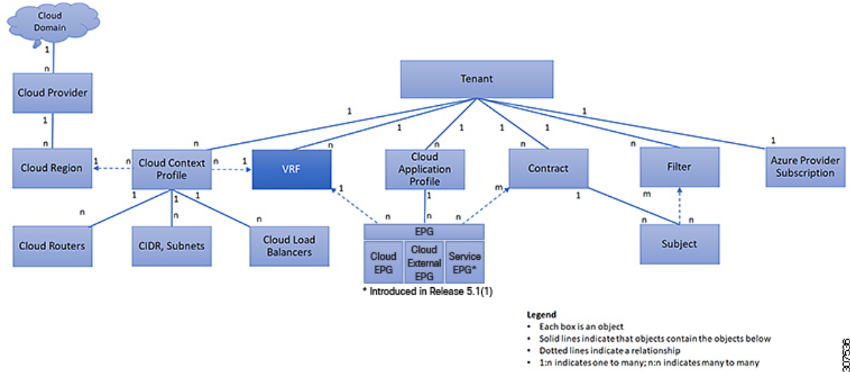
Figure 14: VRFs
