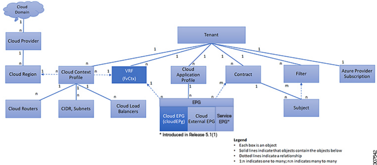
Figure 20: MO Relations
