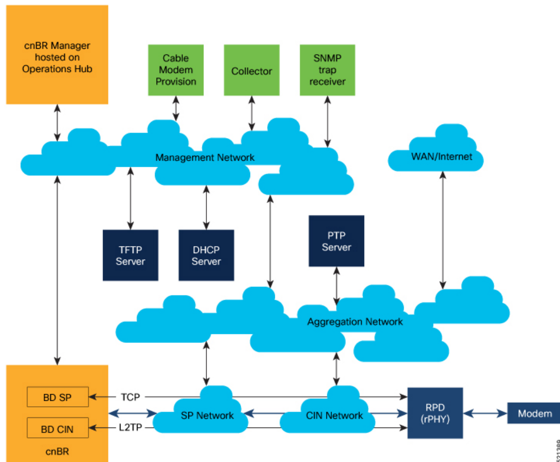
Figure 3: Network Components
