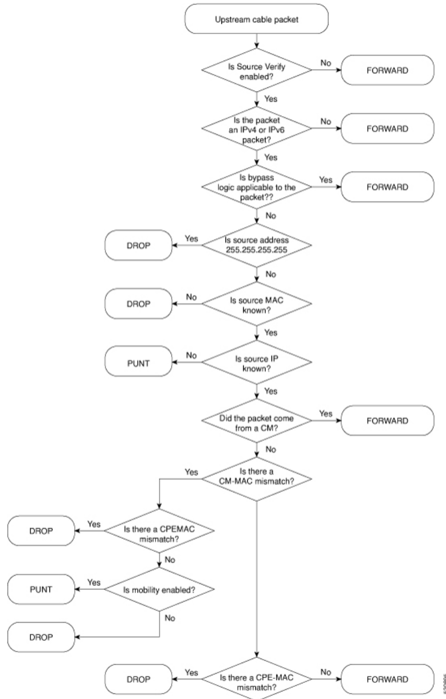
Figure 39: Source-verify logic
