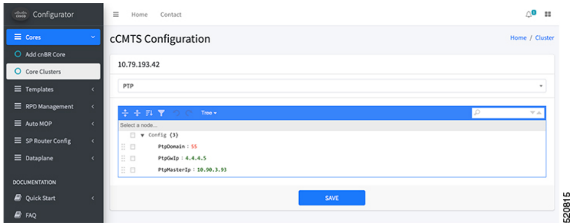
Figure 18: Configuring cnBR PTP Client with a Single Primary Clock
