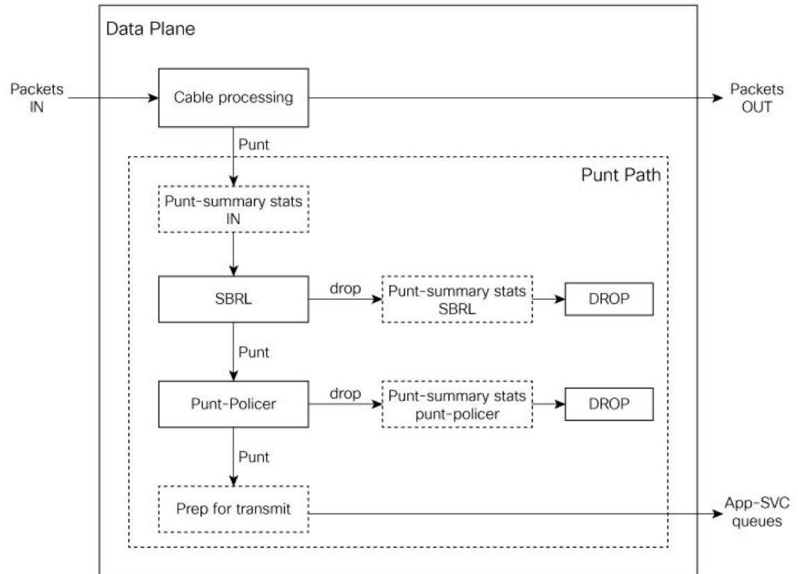
Figure 31: Punt path rate-limiting
