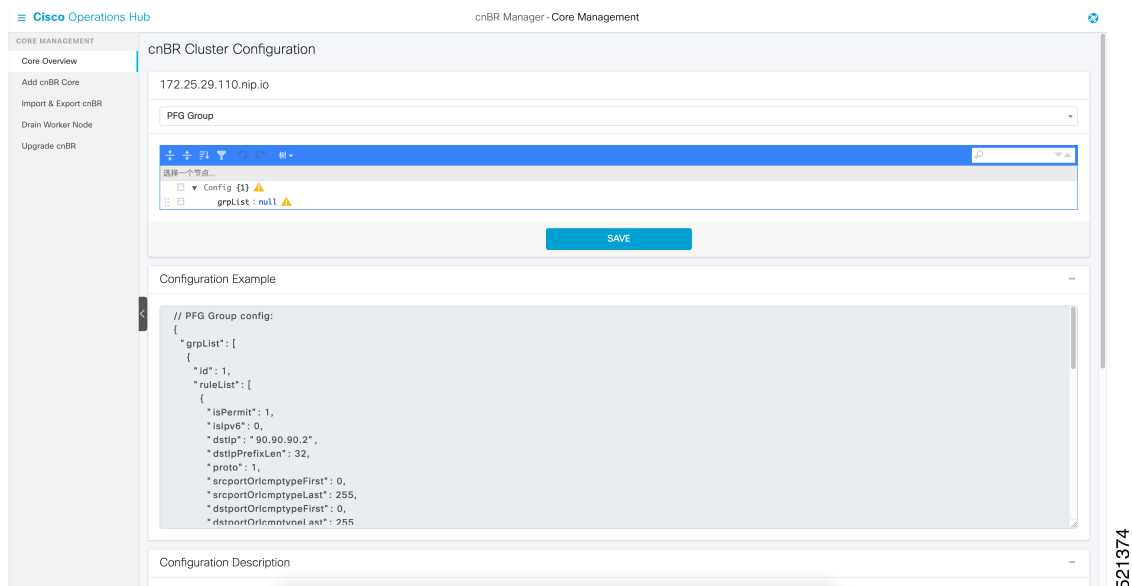
Figure 38: PFG Group Configuration
