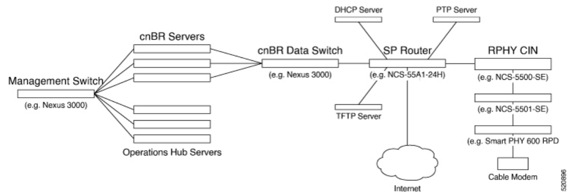
Figure 7: Simplified cnBR Topology
