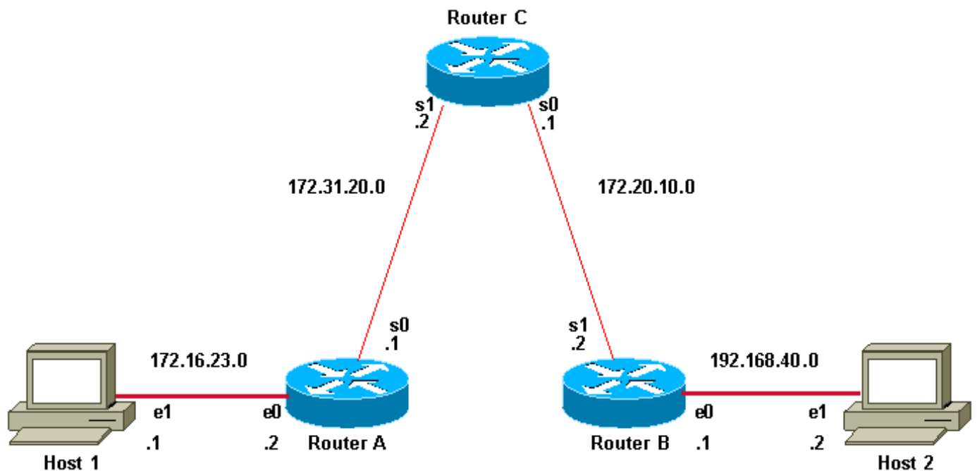
Host 1 and Host 2 cannot Ping
