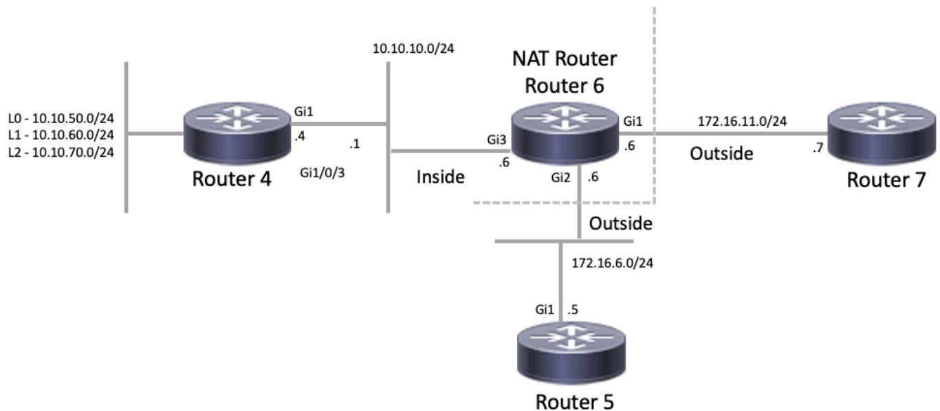
NAT Topology
