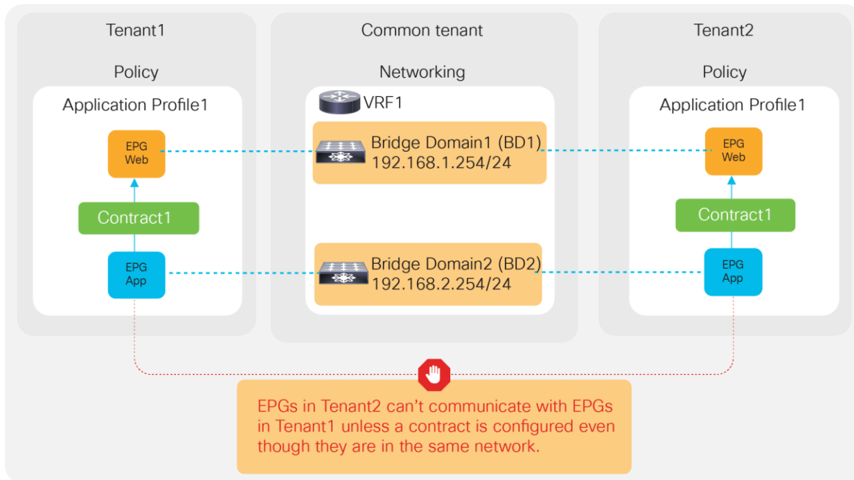
Figure 27. Use of common VRFs/BDs still provides security isolation
