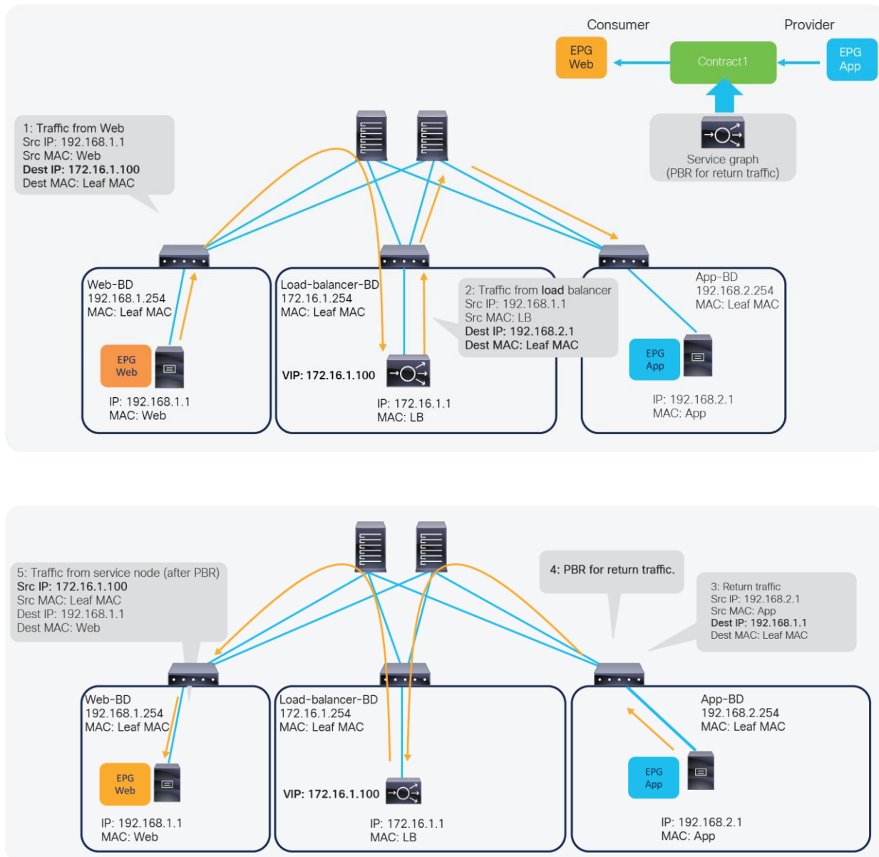
Figure 5. ACI Service Graph PBR use case for load balancer design
