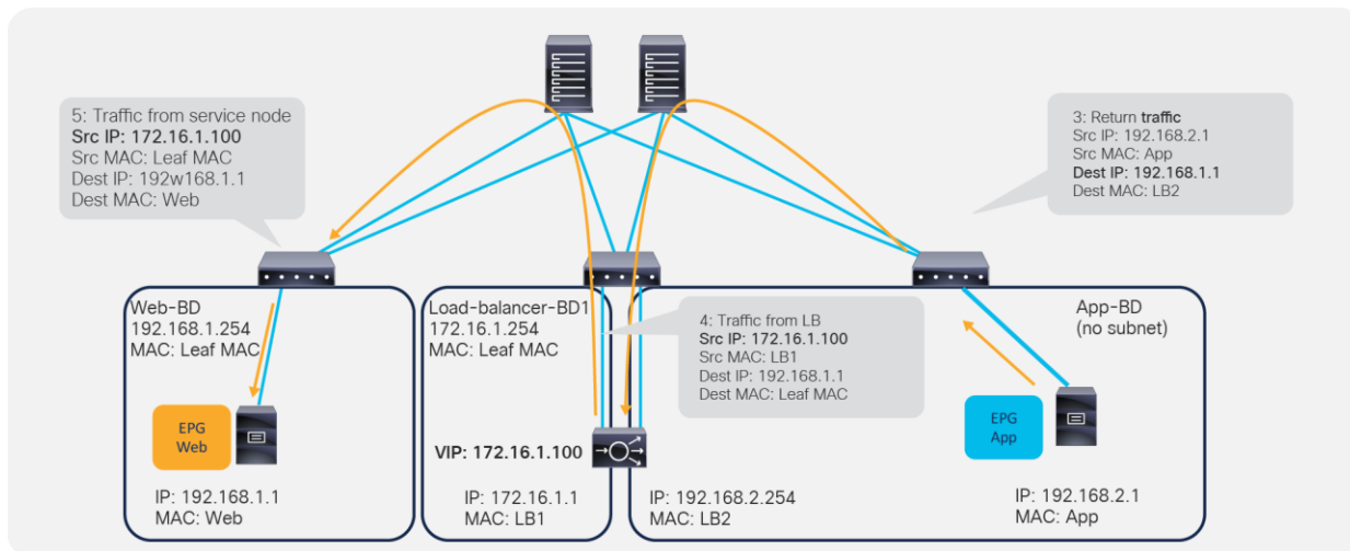
Figure 4. Load balancer design without SNAT or PBR
