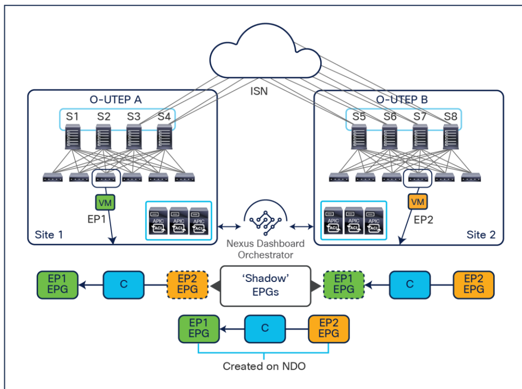
Figure 7. Creation of shadow EPGs
