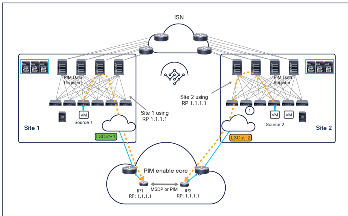
Figure 79. Anycast RP deployment in the external Layer 3 network
