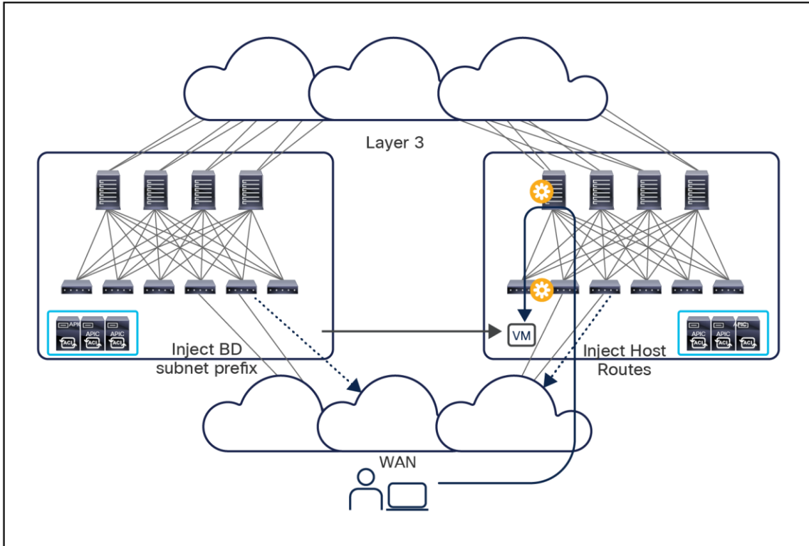
Figure 52. Host-route advertisement on border leaf L3Outs
