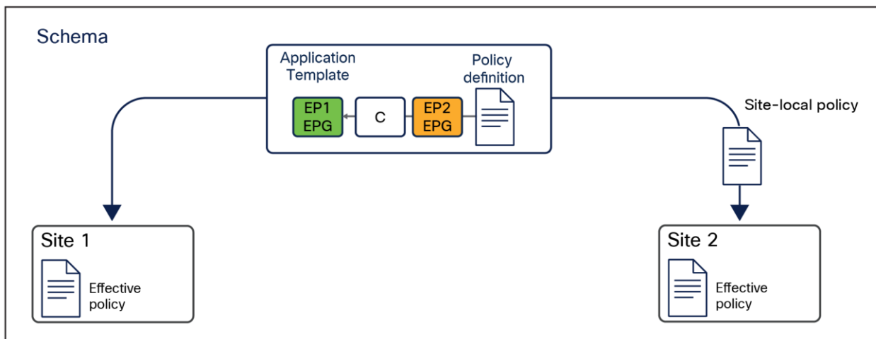
Figure 16. Schema, templates and sites
