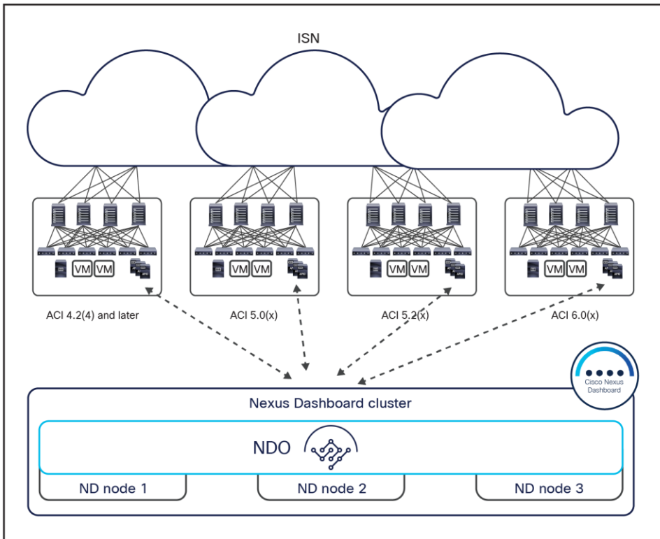
Figure 37. Inter-version support with Cisco Nexus Dashboard Orchestrator releases
