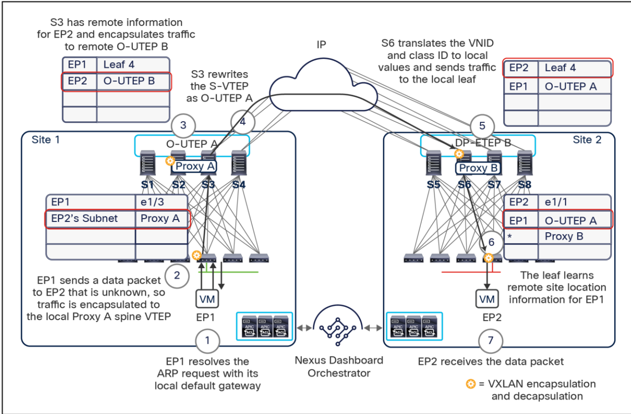
Figure 76. Delivering inter-subnet traffic across sites
