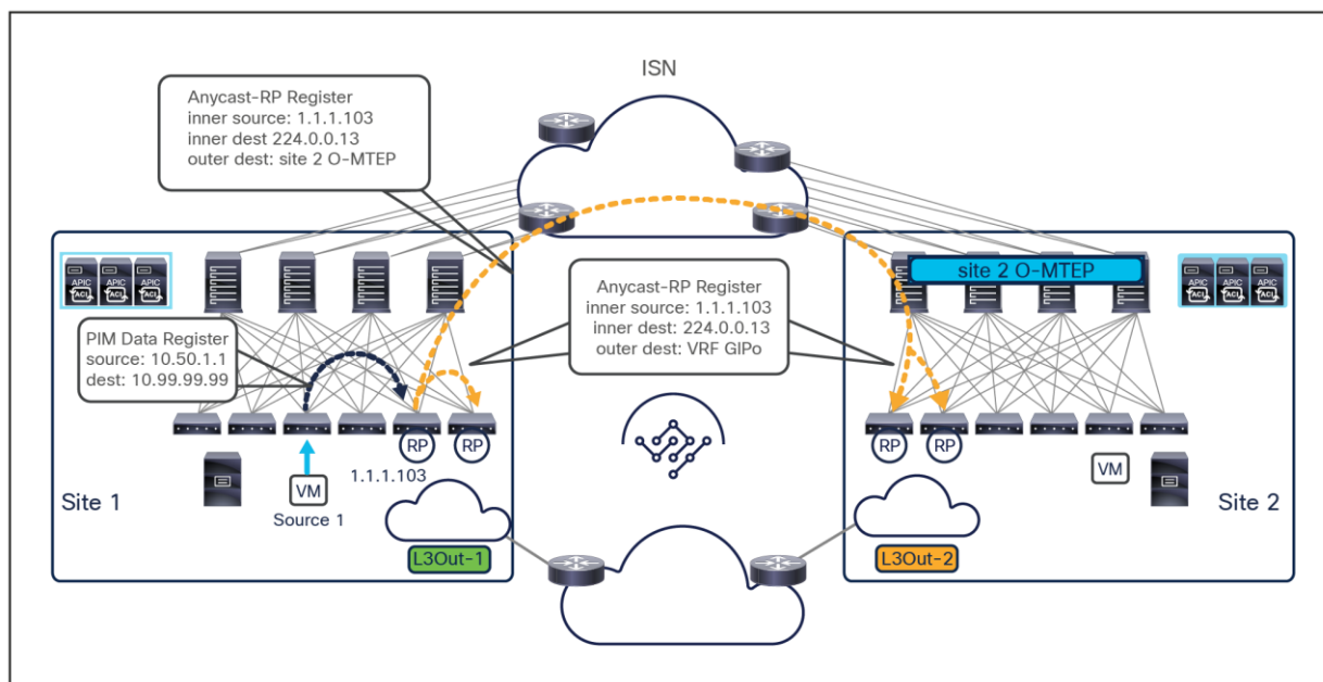
Figure 80. Use of fabric RP in a Multi-Site deployment
