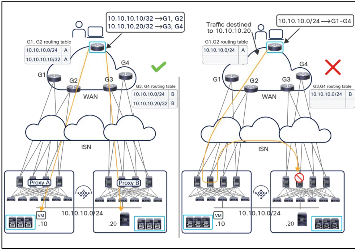
Figure 137. Ingress traffic drop without host-route advertisements on GOLF L3Outs
