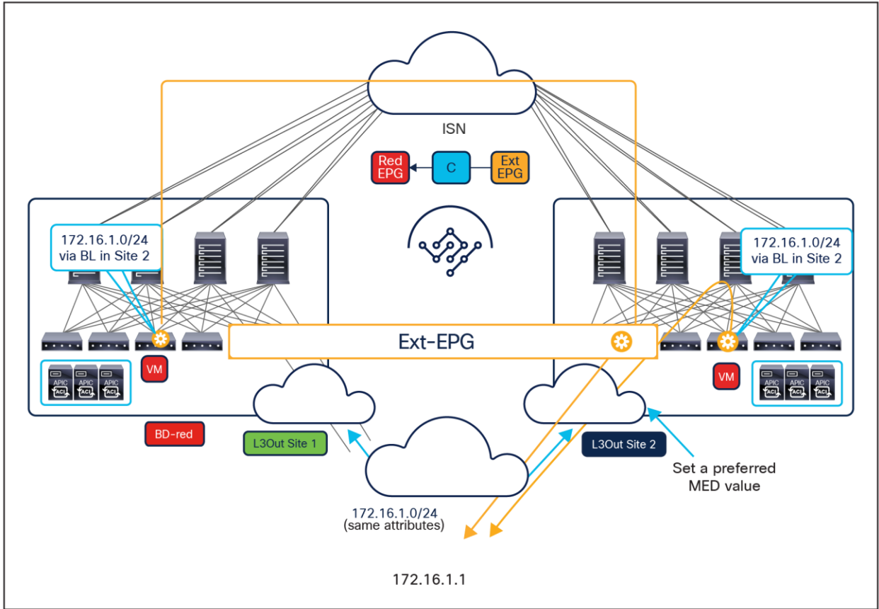
Figure 117. Forcing outbound traffic through a specific L3Out
