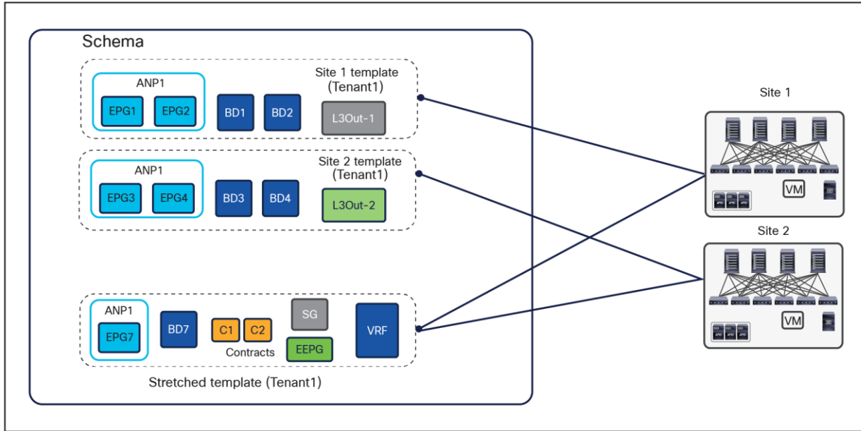
Figure 29. Best practices to define application templates inside a schema with NDO 3.x releases
