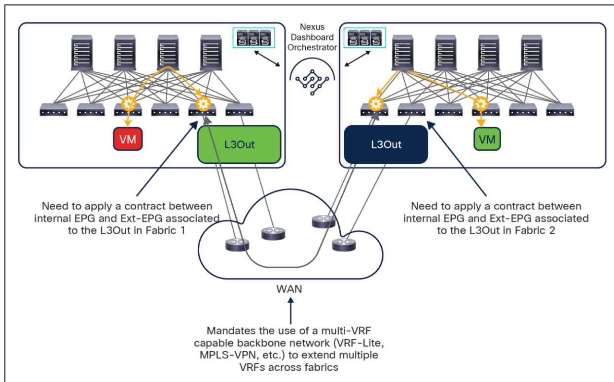
Figure 45. Interconnecting Cisco ACI fabrics for Layer 3 communication via L3Outs
