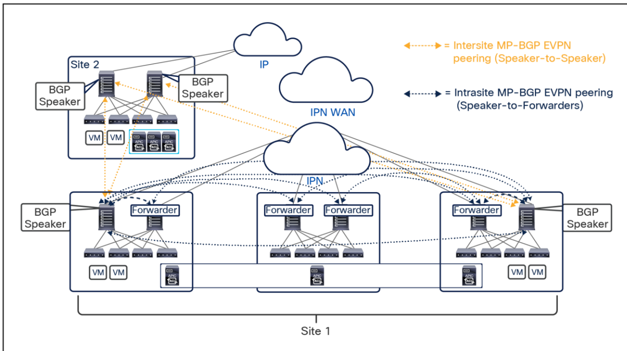
Figure 93. Hierarchical MP-BGP EVPN peering
