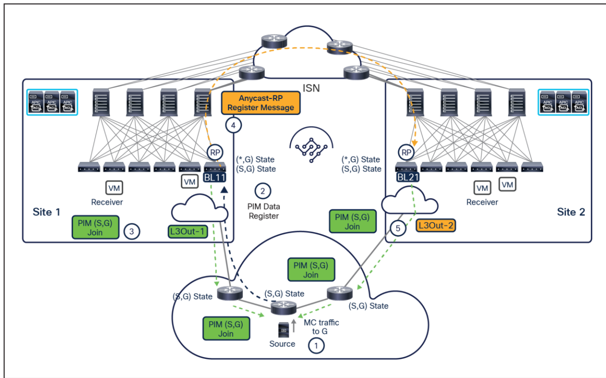
Figure 85. Control plane activity when an external source starts streaming traffic to multicast group G
