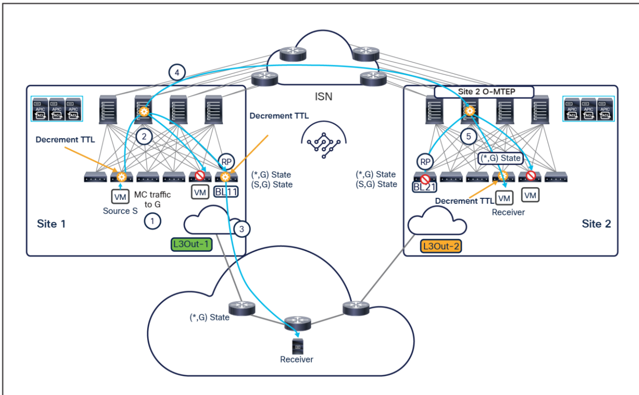
Figure 83. Data-plane forwarding of the multicast stream toward remote and external receivers
