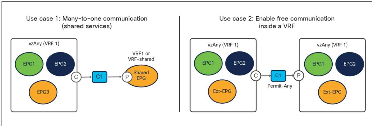
Figure 12. Main use cases supported with vzAny
