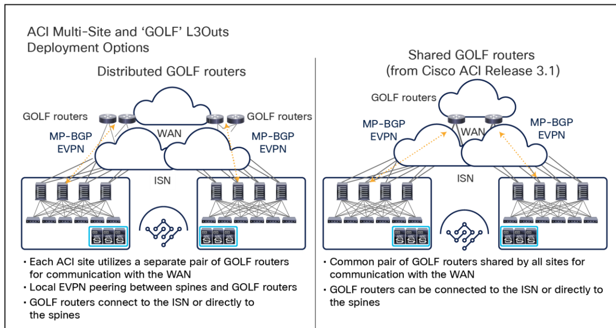
Figure 133. Dedicated or shared pairs of GOLF routers
