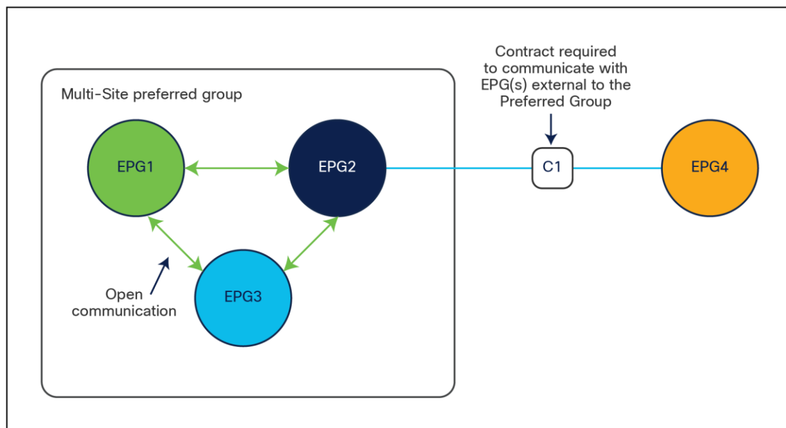
Figure 10. EPGs and preferred groups
