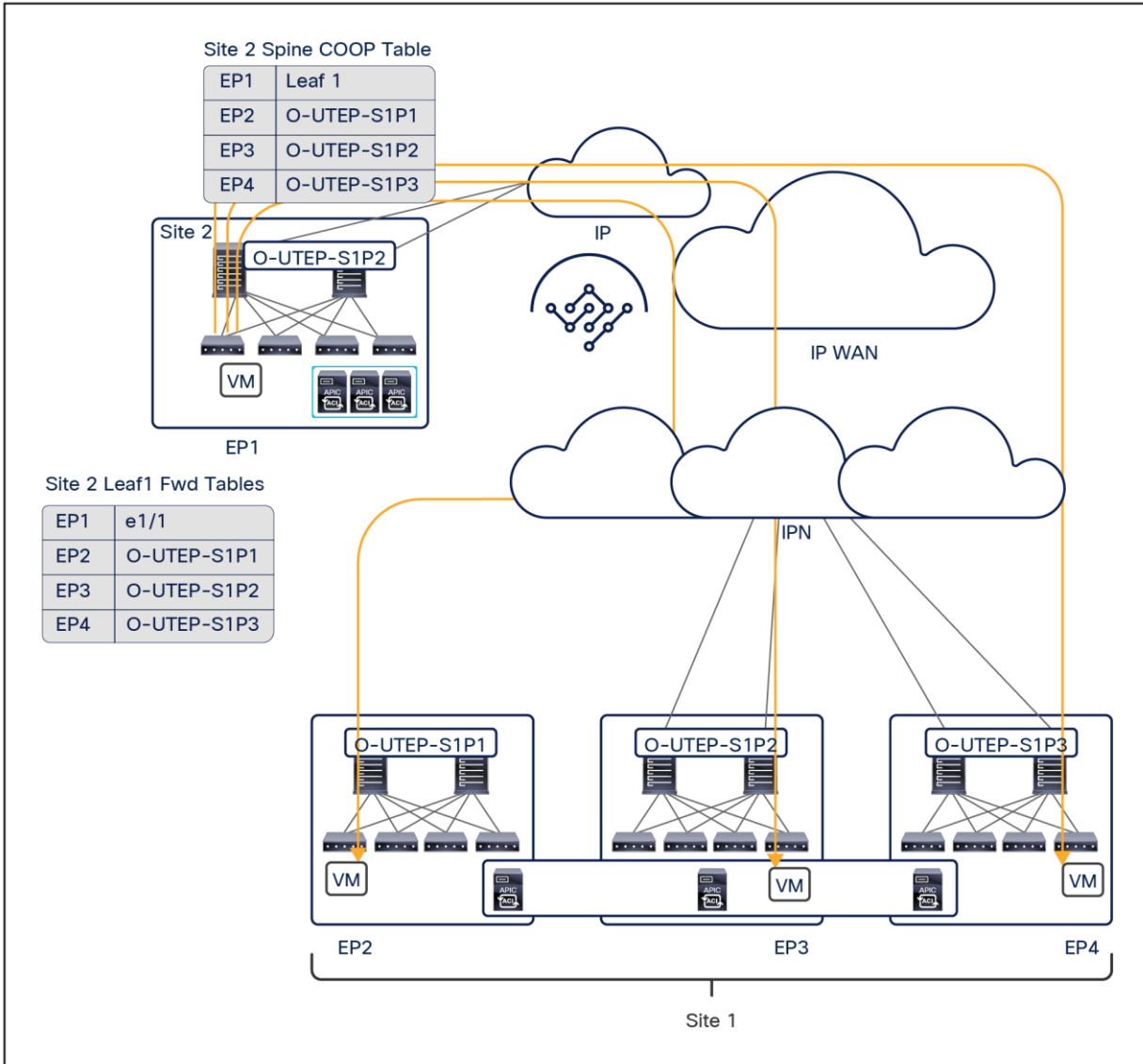
Figure 94. Unicast traffic ingress a Multi-Pod fabric that is part of Cisco ACI Multi-Site
