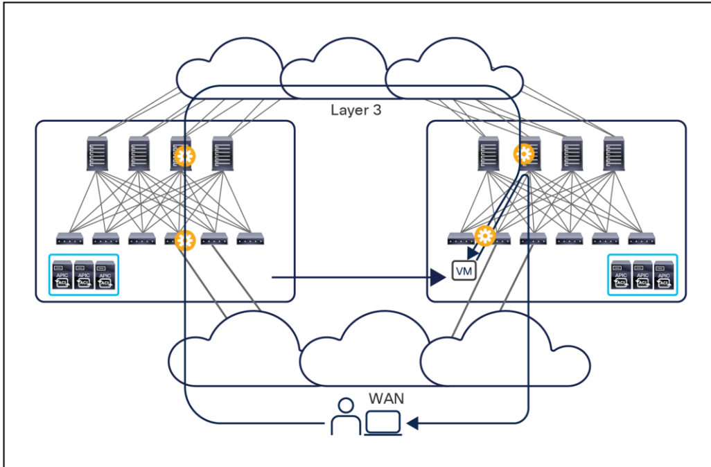
Figure 51. Bouncing traffic across sites toward the migrated endpoint
