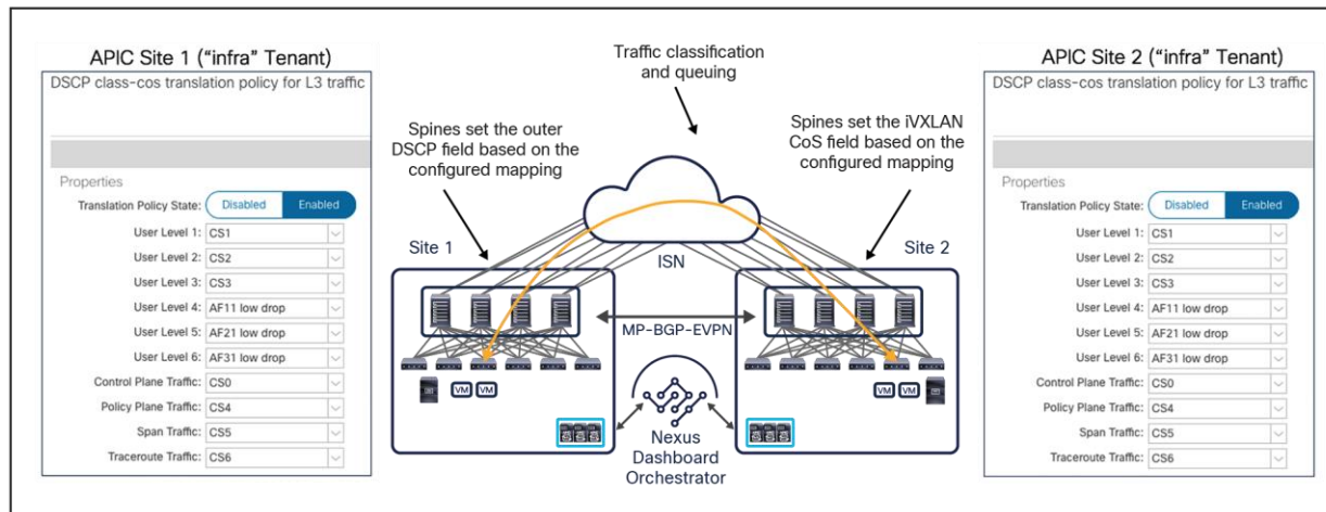
Figure 59. End-to-end consistent QoS behavior between ACI sites
