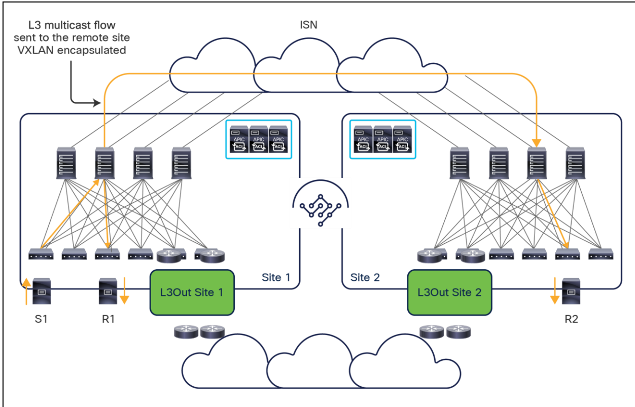
Figure 78. Layer 3 multicast support with Cisco ACI Multi-Site (from Cisco ACI Release 4.0(2))
