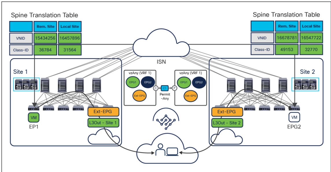
Figure 14. Establishment of any-to-any intra-VRF communication
