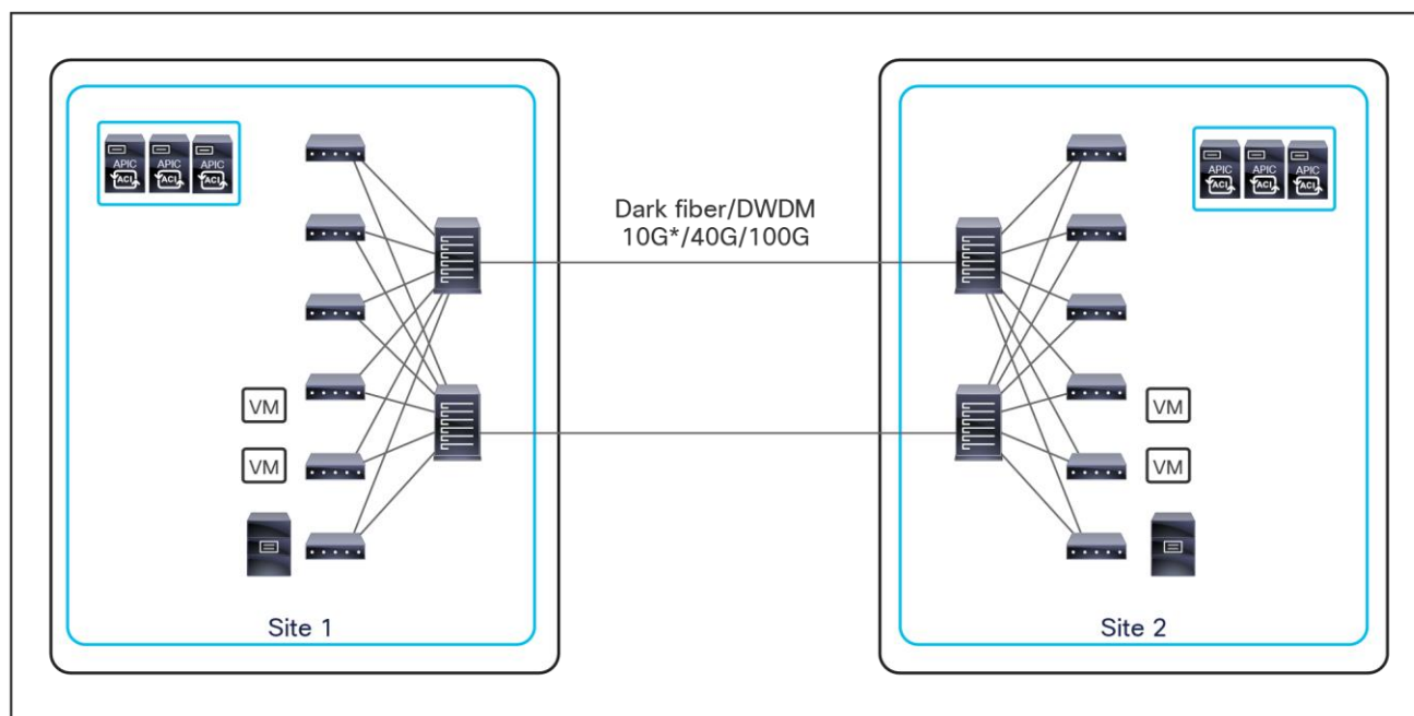
Figure 62. Cisco ACI Multi-Site spines back-to-back connectivity (from Cisco ACI Release 3.2)
