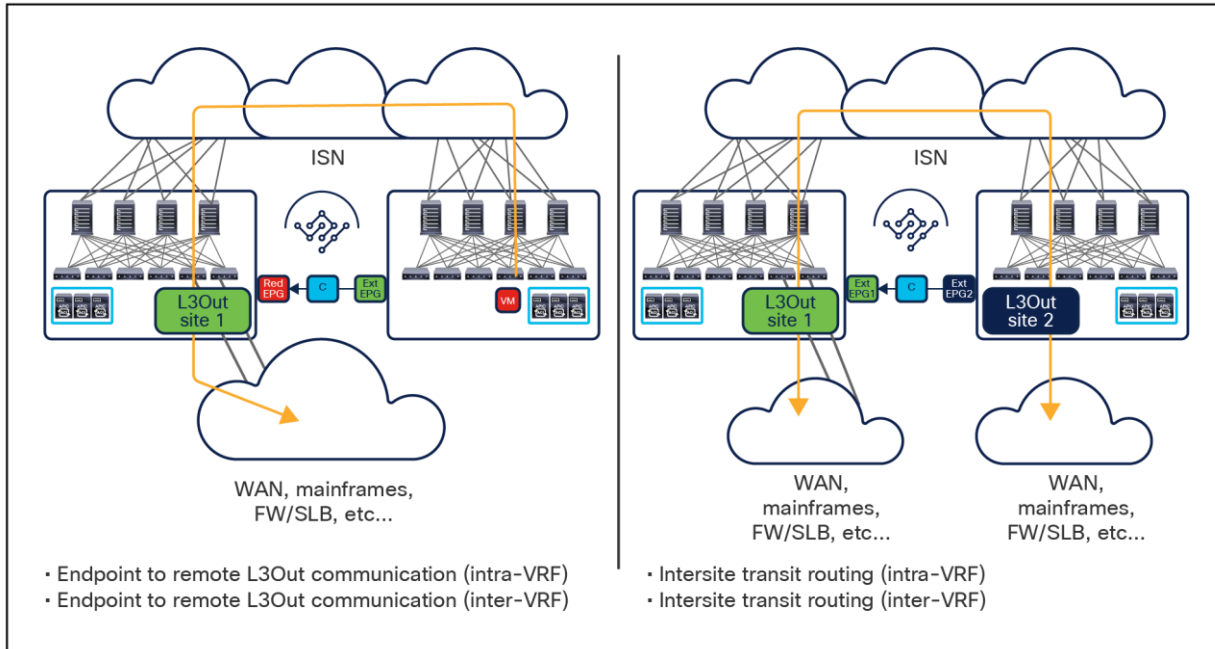
Figure 108. Use cases supported with Intersite L3Out functionality
