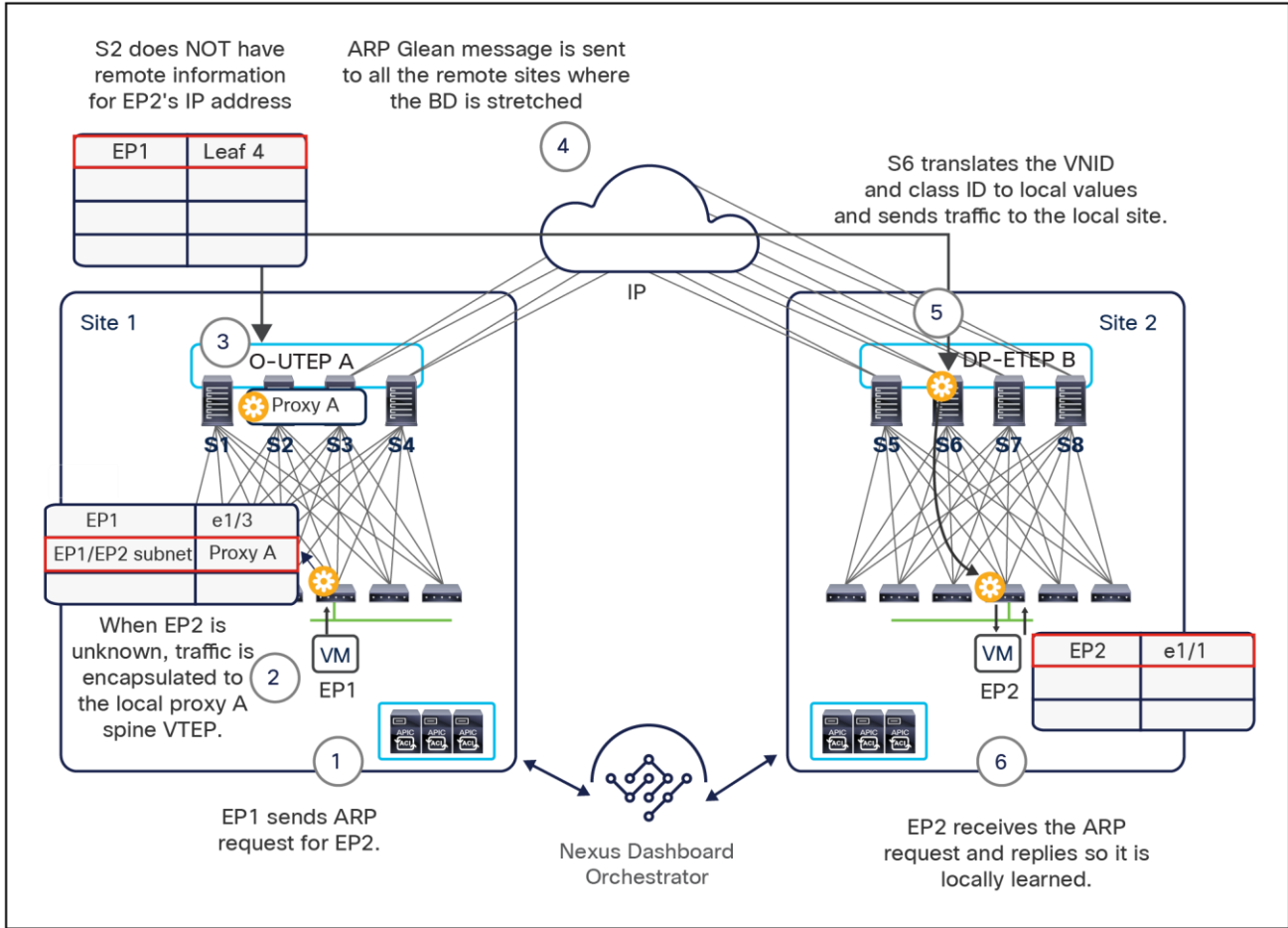
Figure 73. ARP Glean functionality for intra-subnet communication use case
