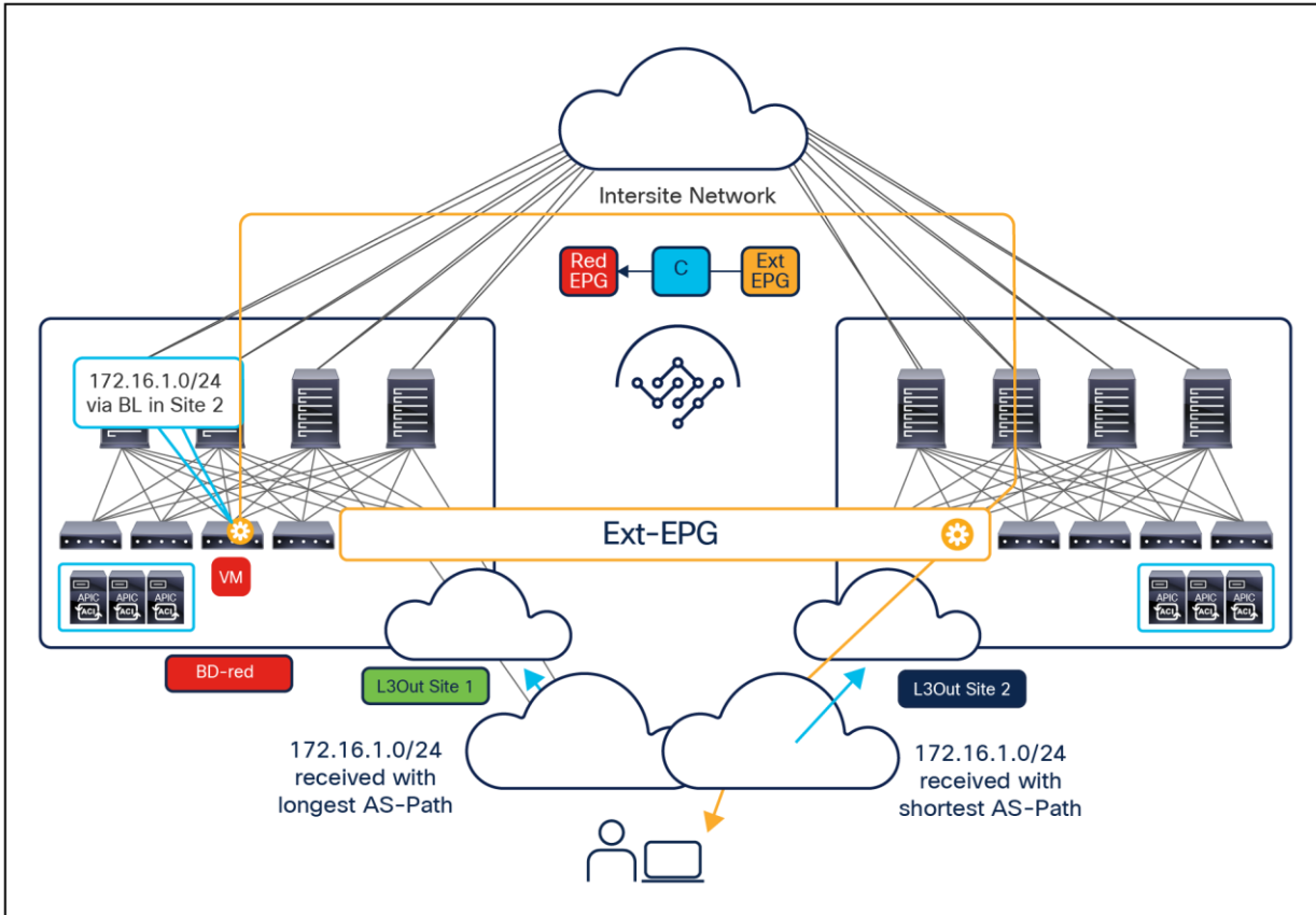
Figure 115. Suboptimal outbound traffic path
