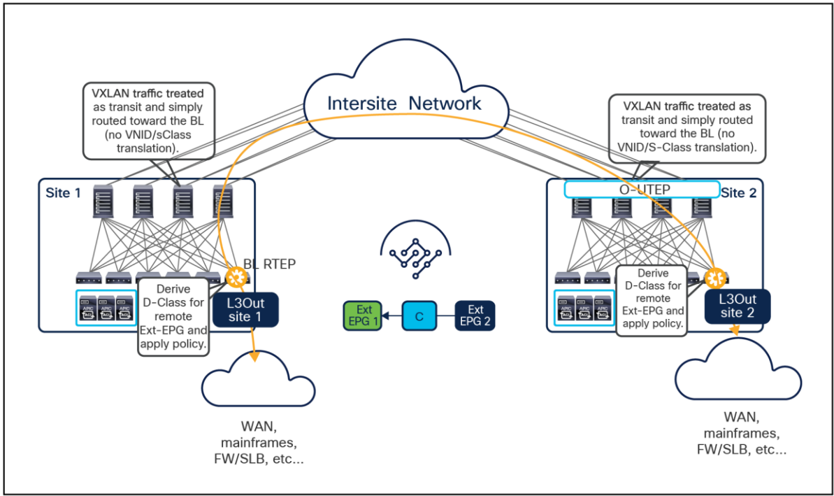
Figure 113. Transit routing across ACI sites
