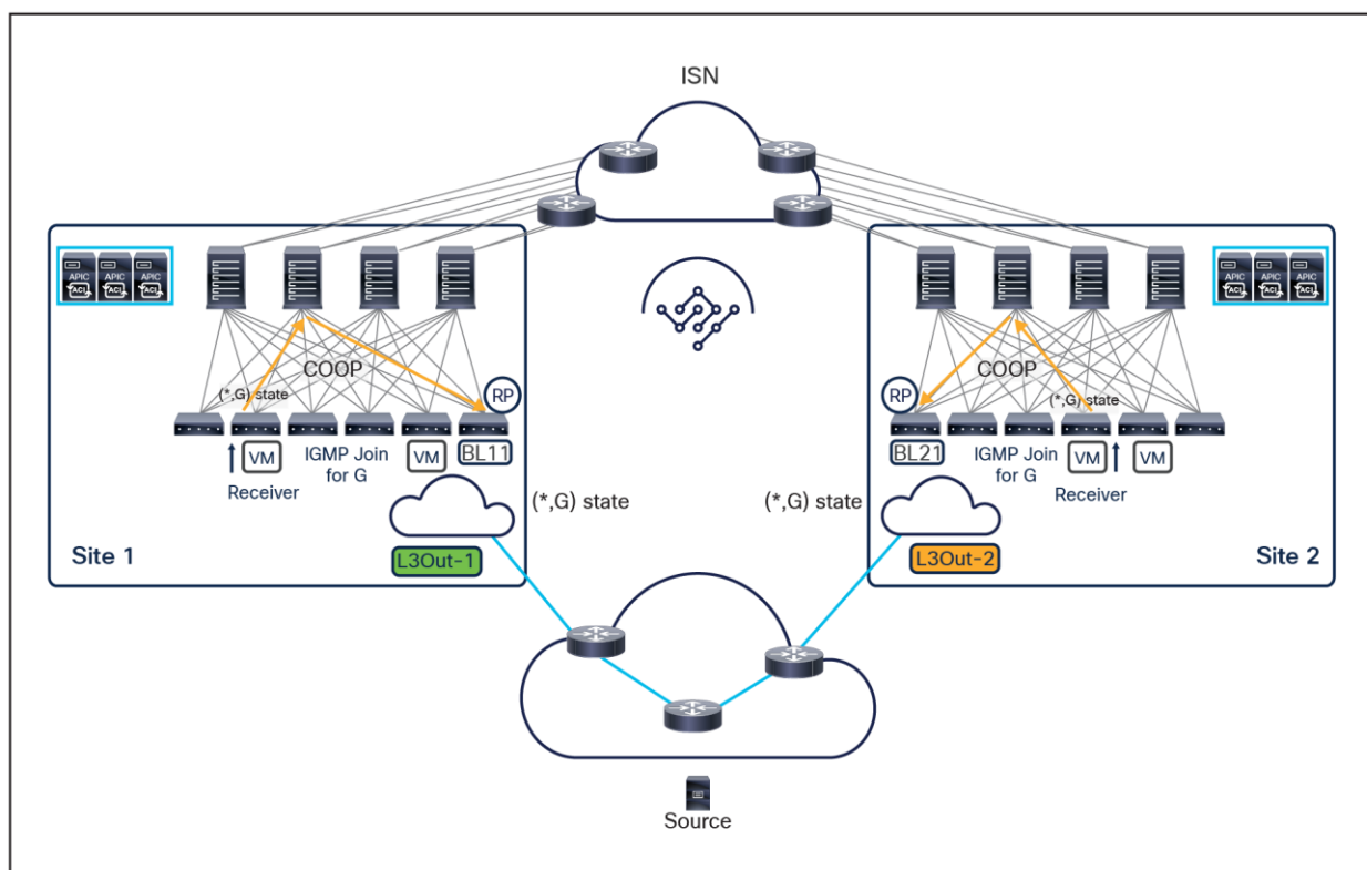
Figure 84. Control plane activity when internal receivers join multicast group G
