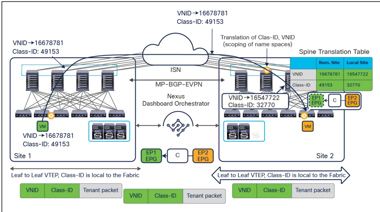
Figure 8. Name-space translation function on the receiving spine
