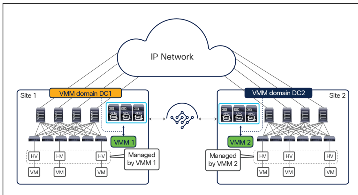
Figure 120. Multiple virtual machine managers across sites
