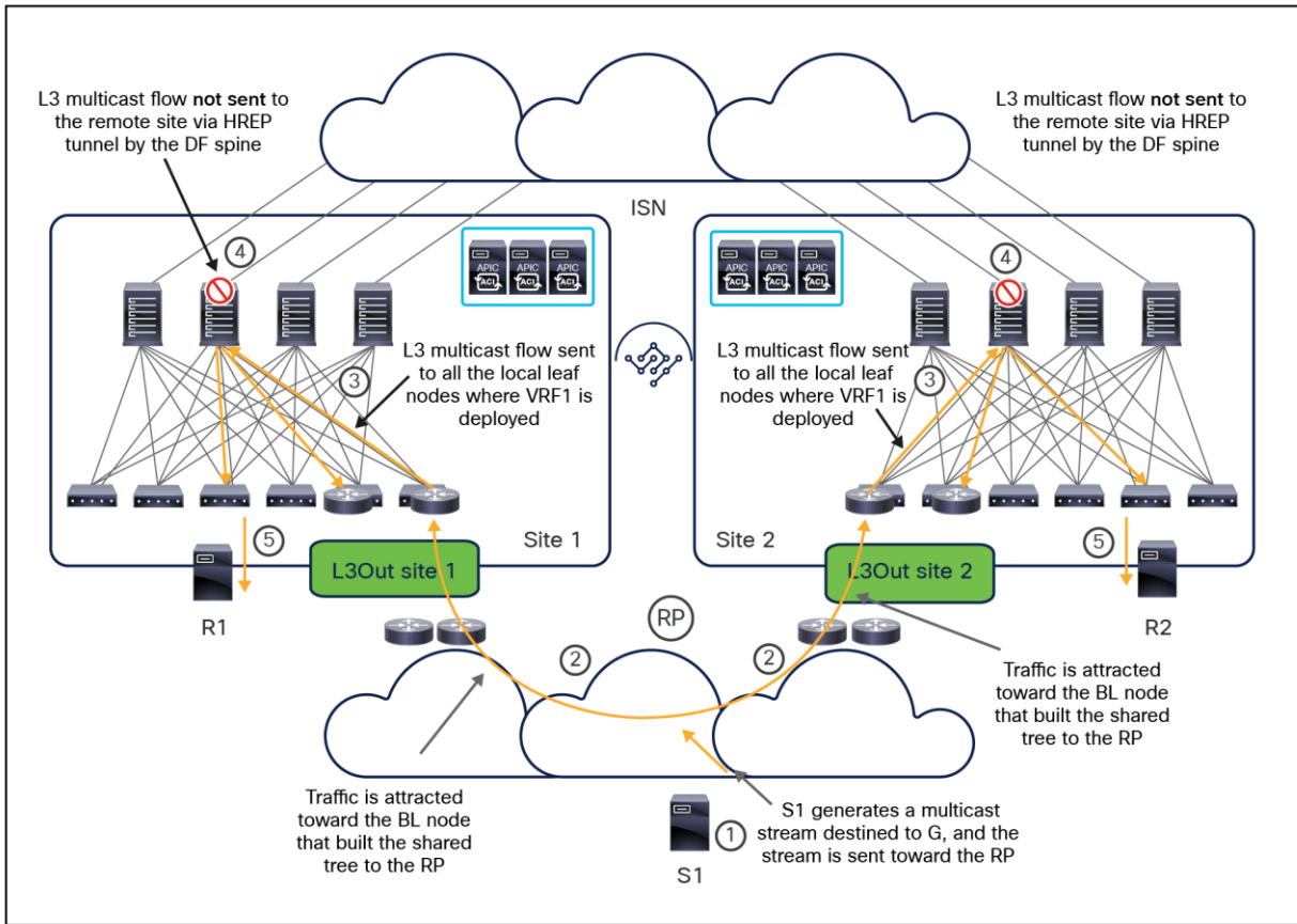
Figure 130. Layer 3 multicast forwarding between external source and internal/external receivers
