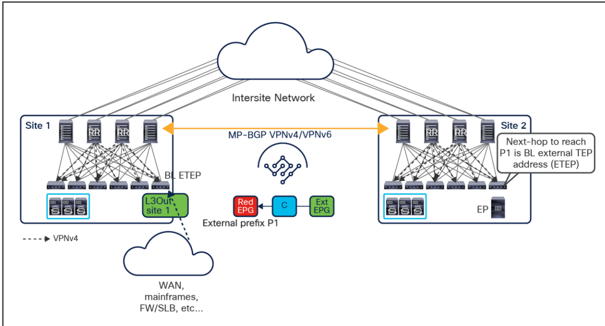
Figure 110. VPNv4/VPNv6 BGP Adjacencies across sites
