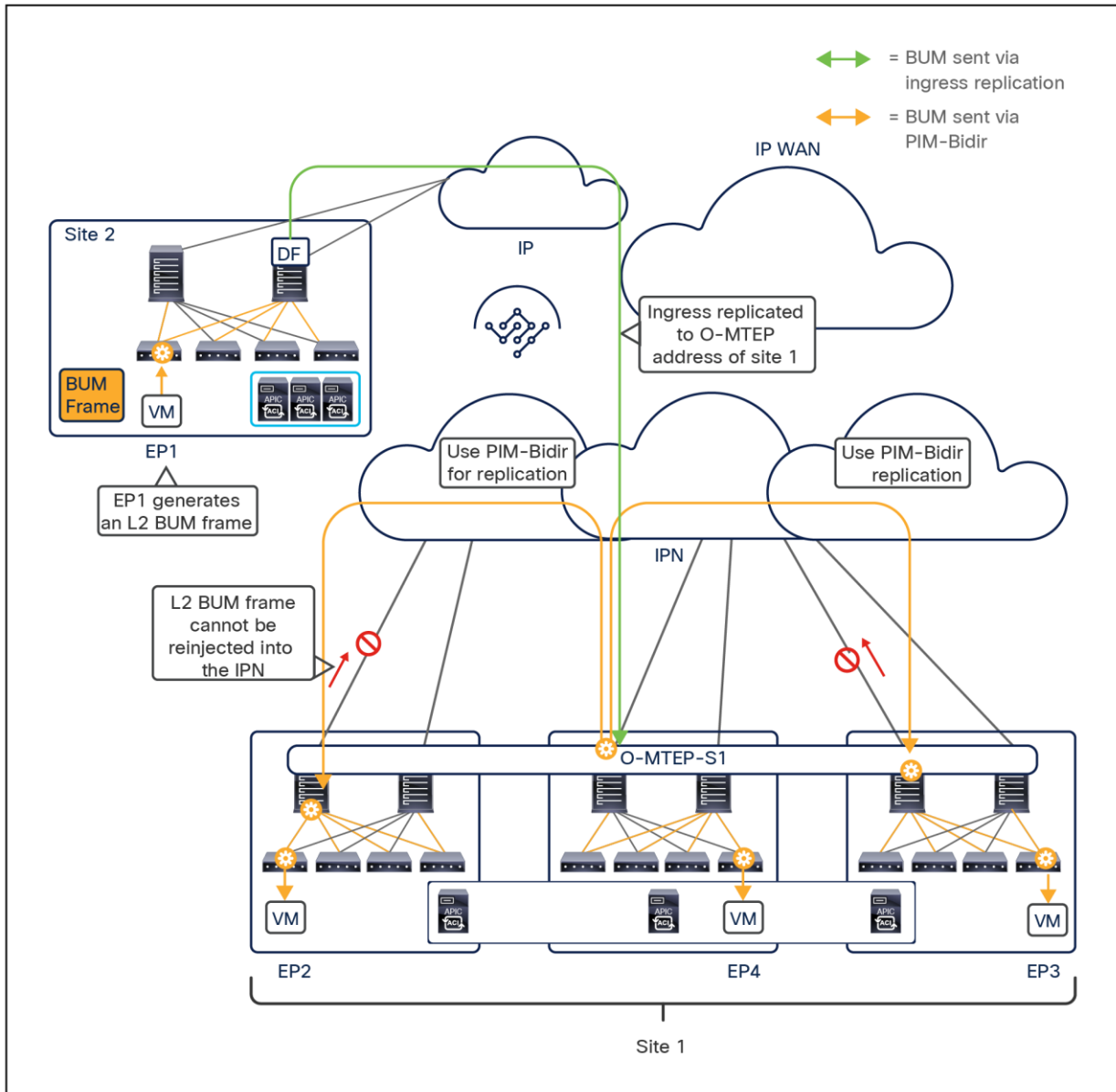
Figure 95. Layer 2 BUM traffic ingressing a Multi-Pod fabric that is part of Cisco ACI Multi-Site
