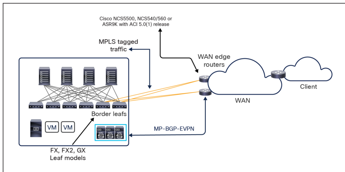
Figure 98. SR-MPLS/MPLS hand-off on border leaf nodes
