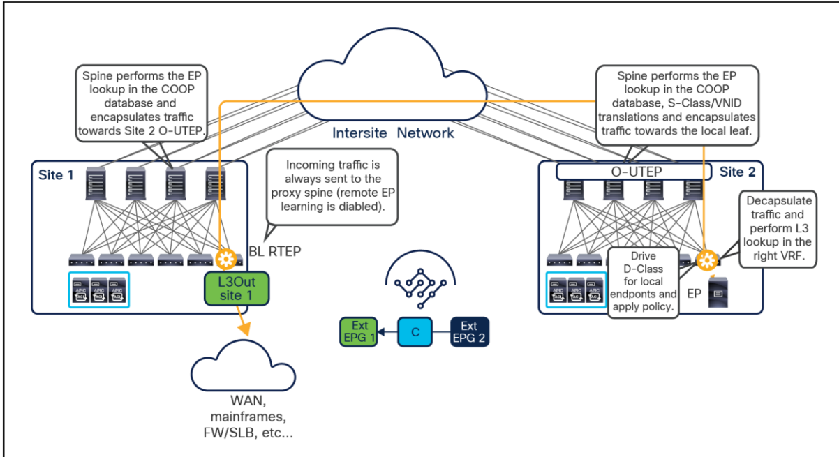
Figure 112. Return traffic from the L3Out to the remote endpoint
