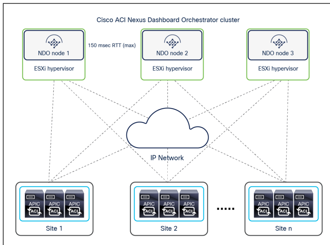
Figure 131. VM-based MSO cluster running on VMware ESXi hosts
