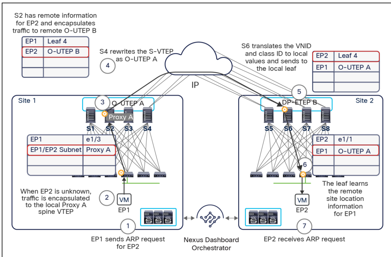
Figure 72. ARP request across sites without flooding
