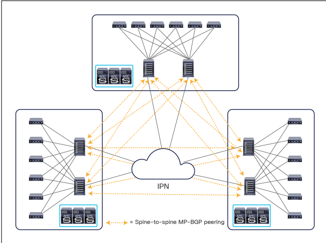
Figure 67. Full mesh of EVPN sessions across sites
