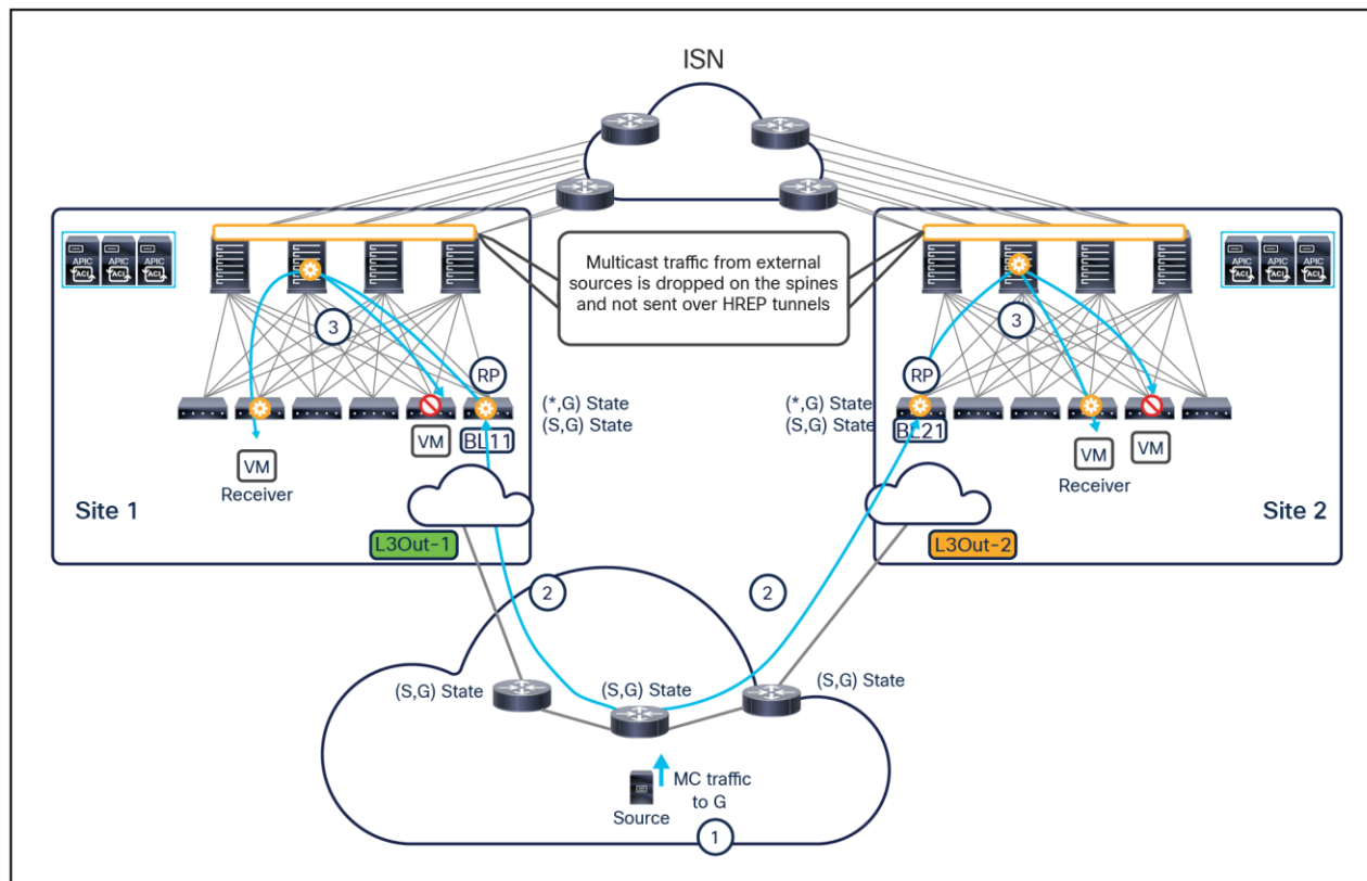
Figure 86. Data-plane forwarding of the multicast stream toward internal receivers
