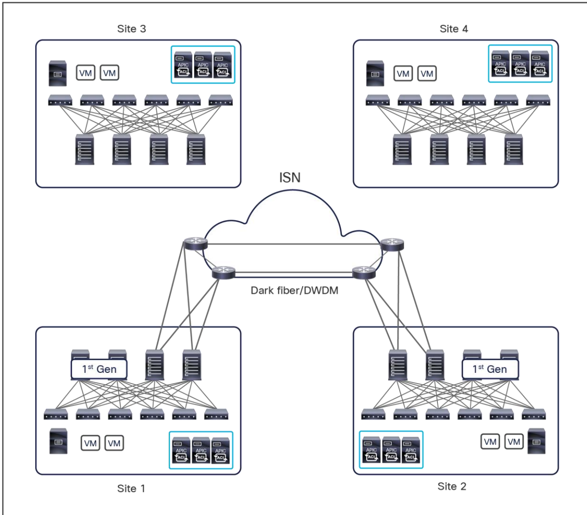
Figure 64. Connecting first-hop ISN routers back to back
