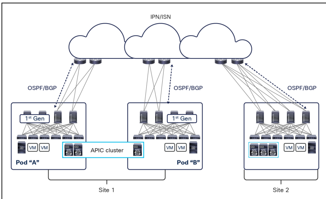
Figure 90. Single network infrastructure offering both IPN and ISN connectivity
