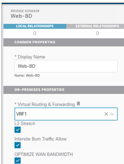
Figure 70. Optimizing BUM flooding across sites
