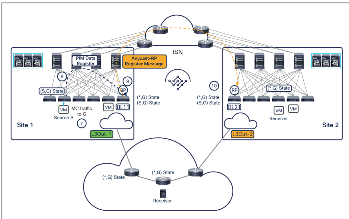
Figure 82. Control plane activity when an internal source starts streaming traffic to multicast group G
