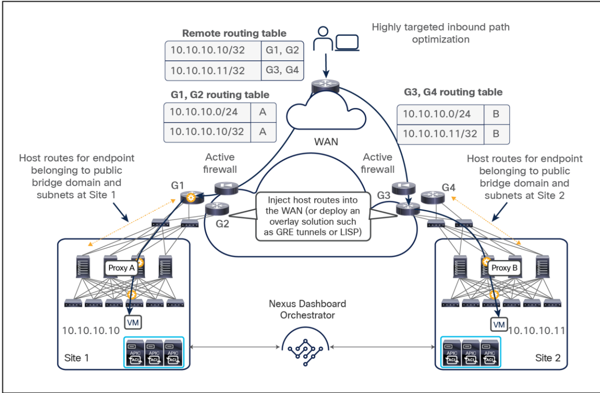
Figure 136. Ingress path optimization using host-route advertisements
