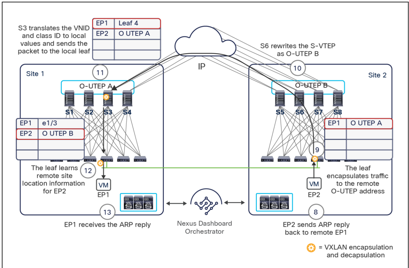
Figure 71. ARP reply delivered to EP1 in site 1
