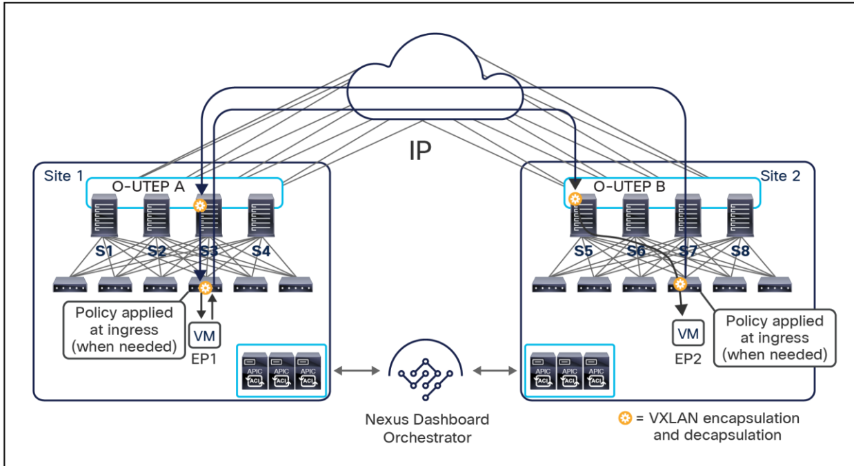
Figure 74. Intra-subnet communication across sites
