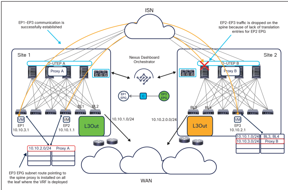
Figure 47. Issue when mixing VXLAN and L3Out traffic paths
