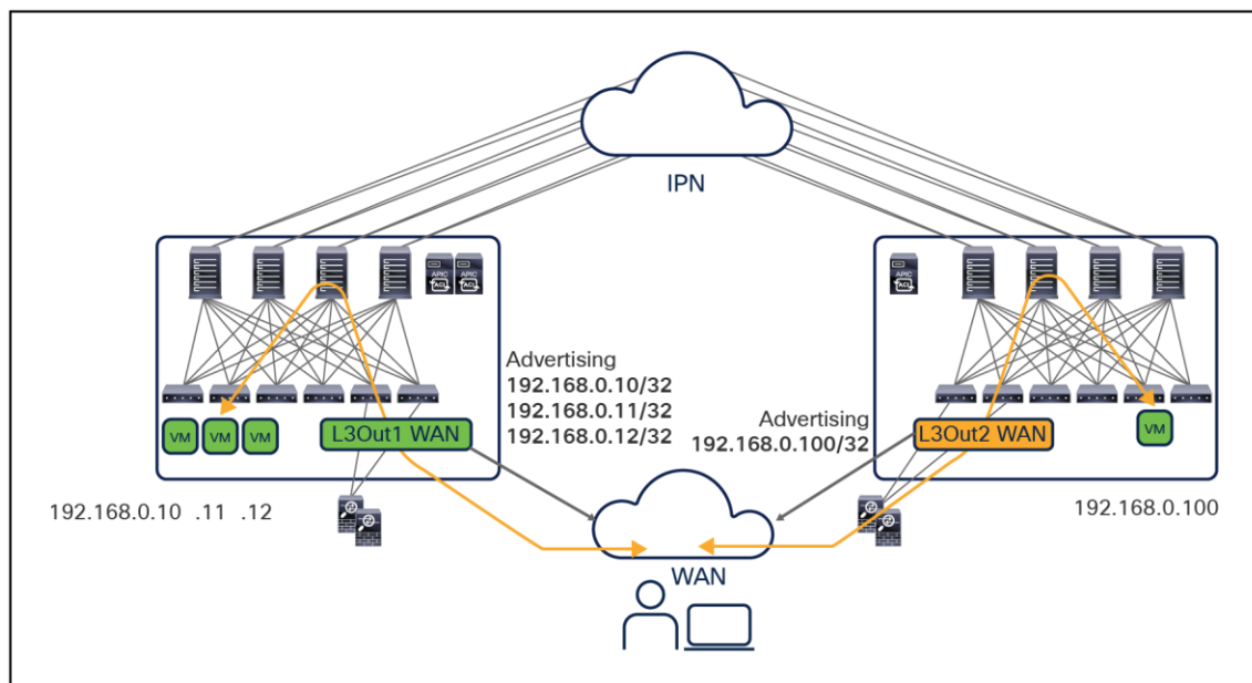
Figure 106. Optimized inbound/outbound traffic flows with host-route advertisement
