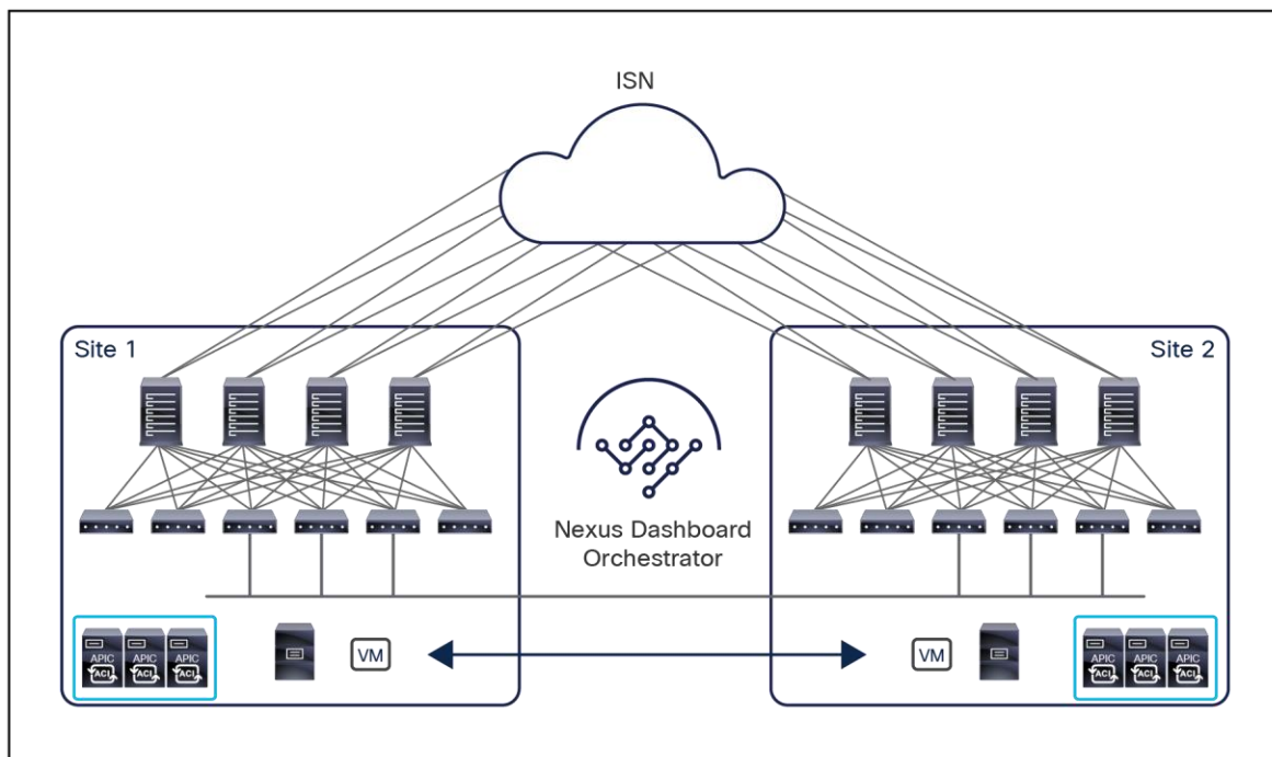
Figure 54. Layer 2 connectivity across sites with flooding
