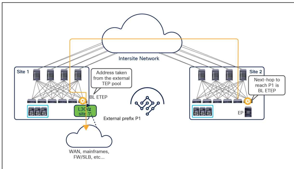
Figure 109. Establishment of leaf-to-leaf VXLAN tunnel across sites
