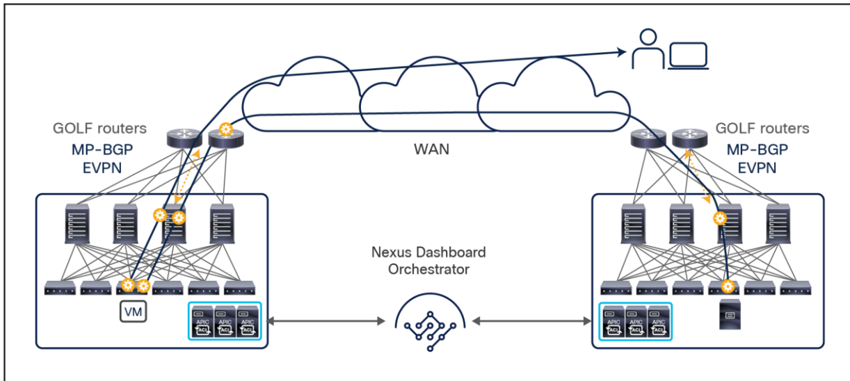
Figure 134. Common Layer 3 infrastructure for east-west and north-south traffic
