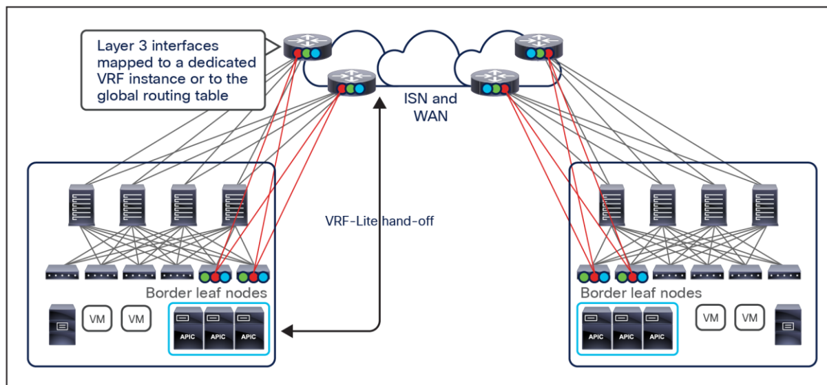
Figure 102. Common Layer 3 infrastructure for east-west and north-south traffic
