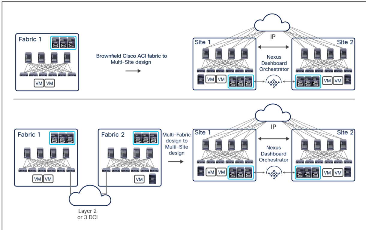
Figure 123. Cisco ACI Multi-Site migration scenarios
