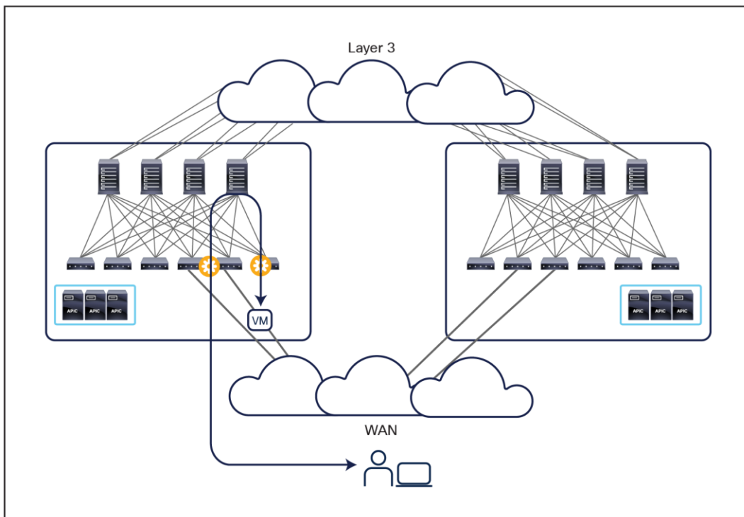
Figure 50. Ingress traffic steered toward the home site
