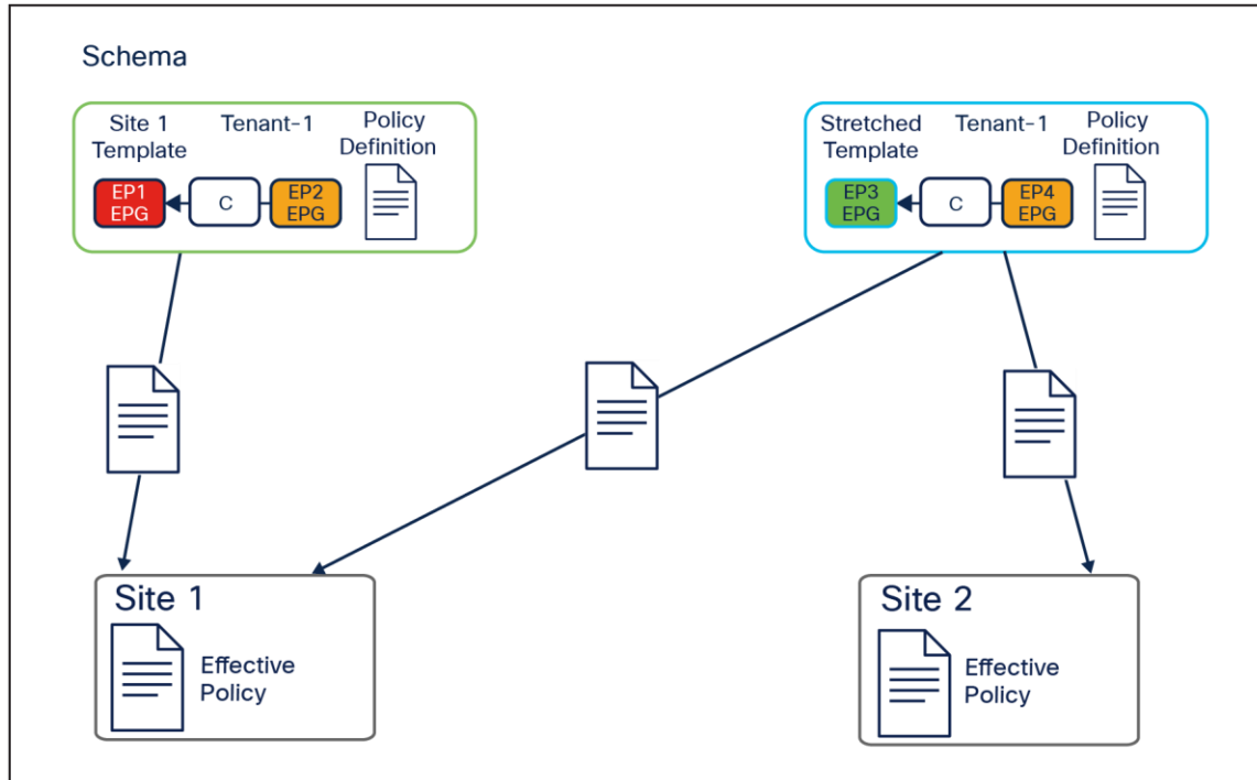
Figure 27. Mapping application templates to ACI sites
