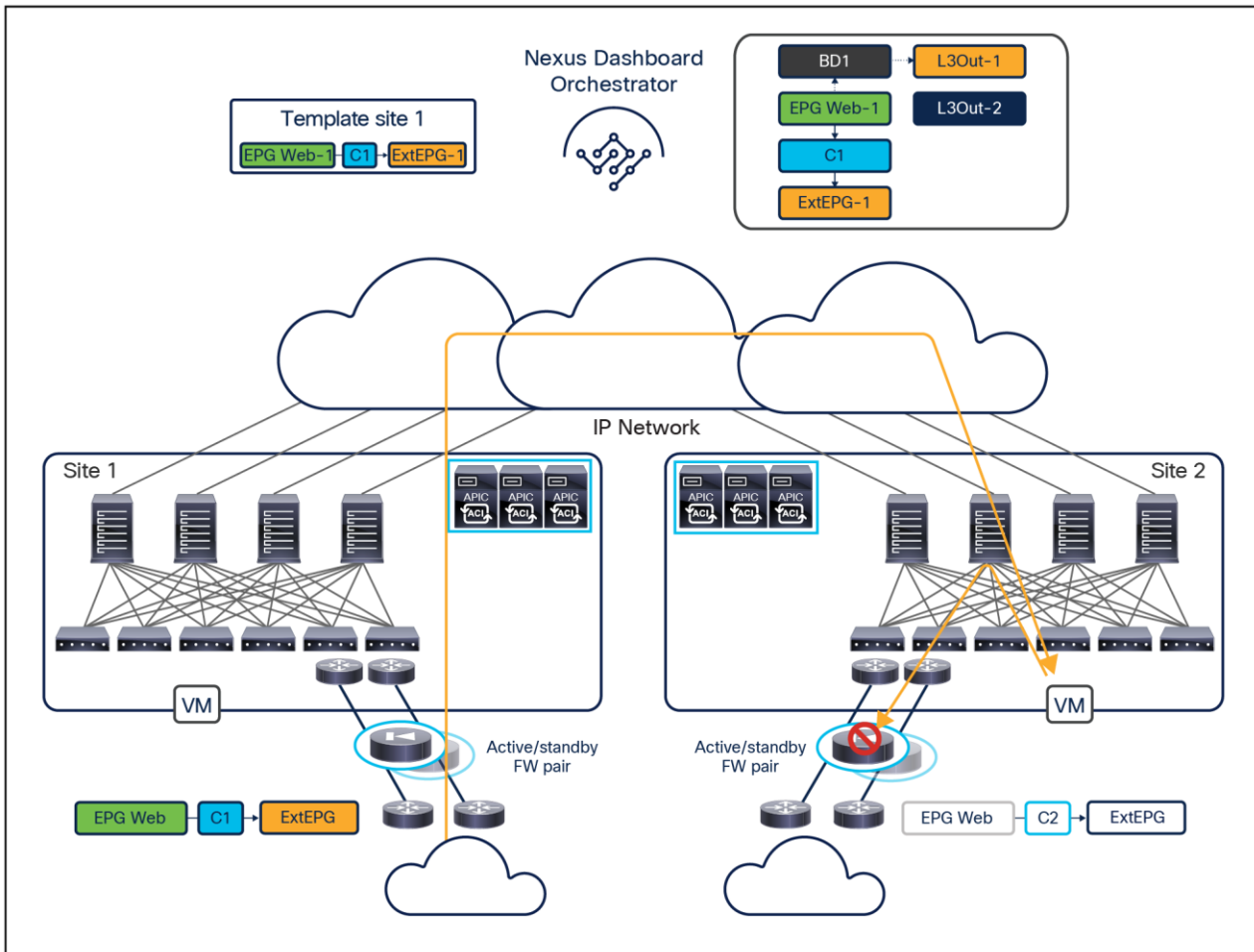
Figure 105. Multi-Site and traditional L3Out connections with a stretched bridge domain
