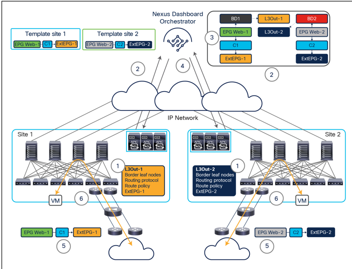
Figure 103. Multi-Site and IP-based L3Out connections on border leaf nodes
