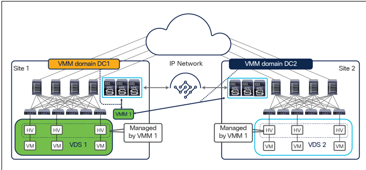
Figure 122. Single VMM with separate VMM domains across sites
