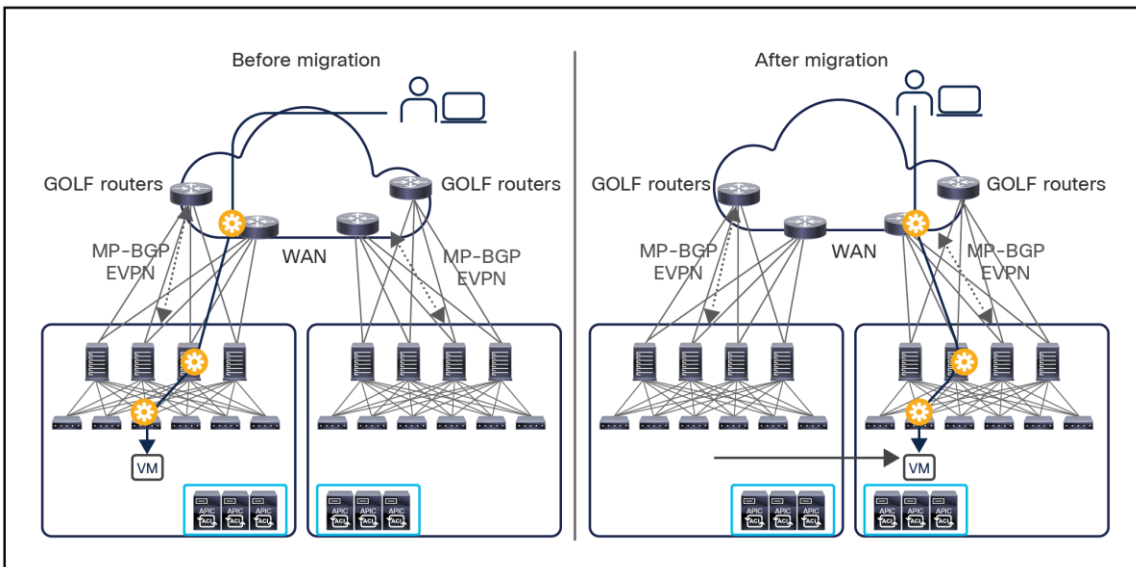
Figure 53. Ingress traffic optimization with GOLF L3Out
