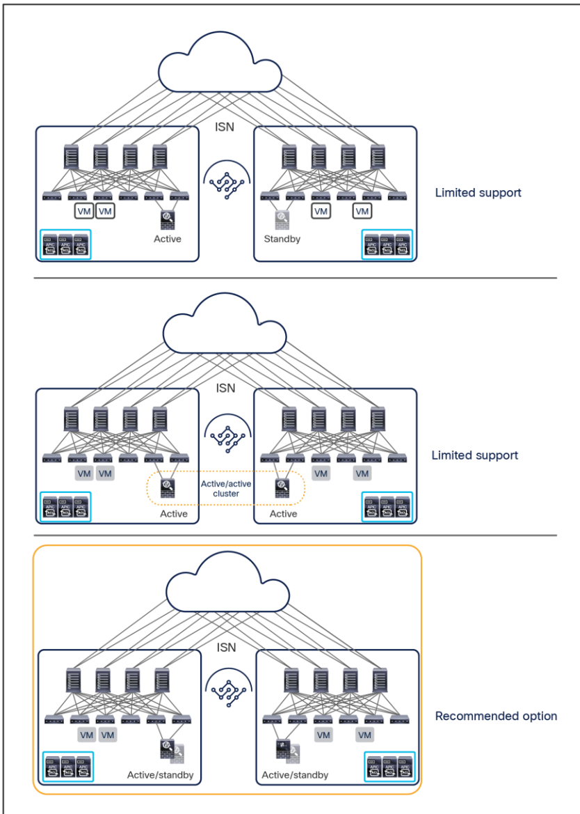
Figure 119. Network-services-integration models with Cisco ACI Multi-Site
