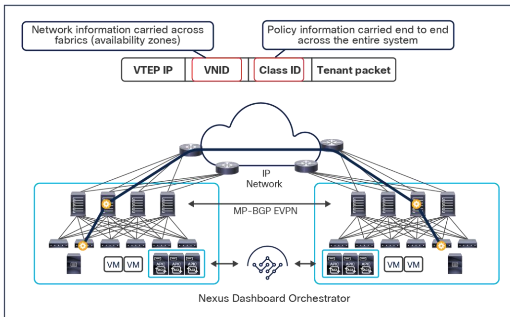
Figure 6. Carrying network and policy information across sites
