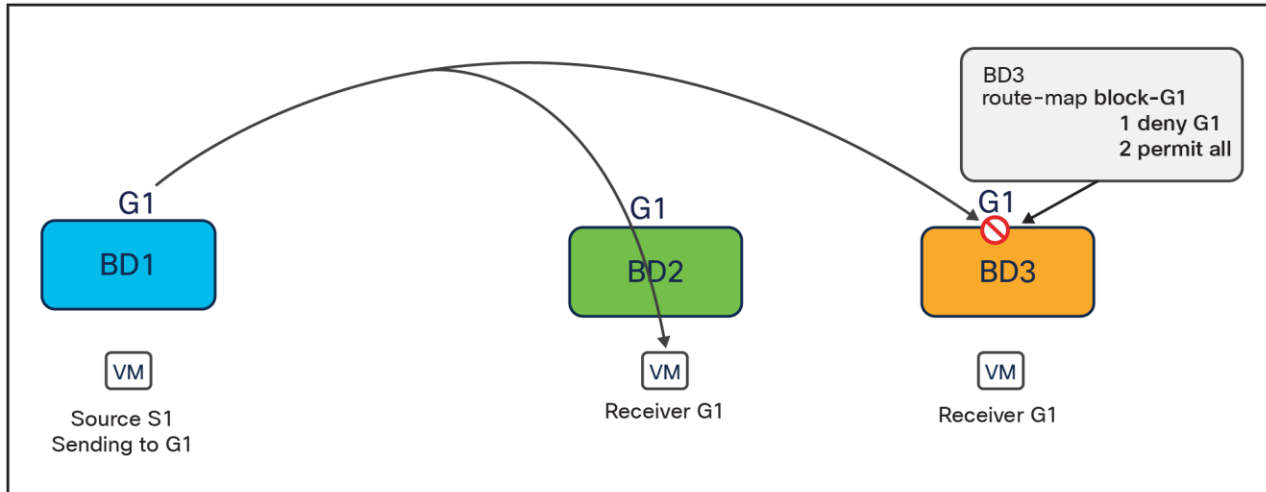
Figure 88. Data plane receiver multicast filtering
