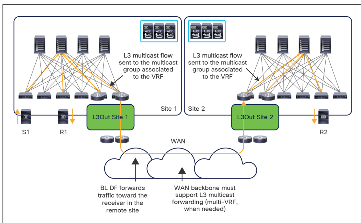
Figure 77. Layer 3 multicast forwarding across separate Cisco ACI fabrics
