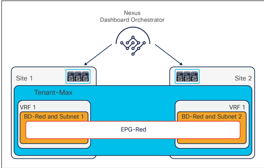
Figure 42. Intra-VRF Layer 3 communication across sites stretching an EPG
