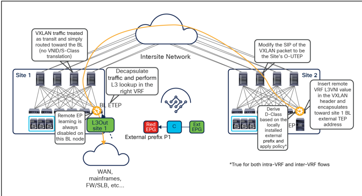
Figure 111. No need for VNID/S-Class translation on the receiving spines
