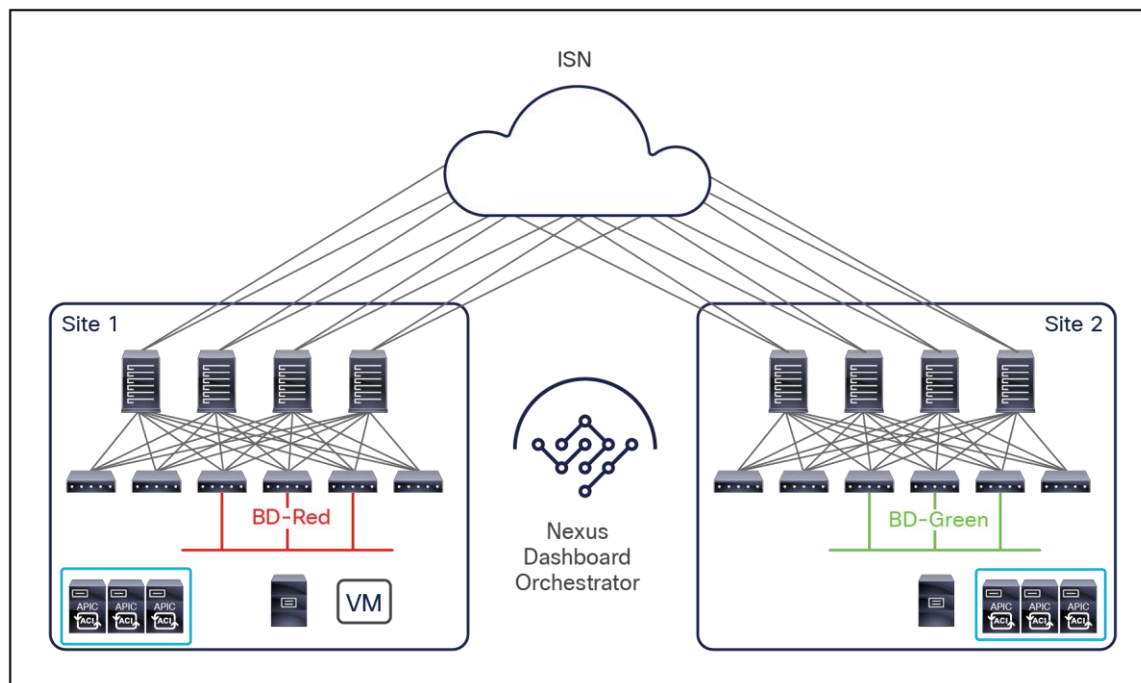
Figure 40. Layer-3-only connectivity across sites
