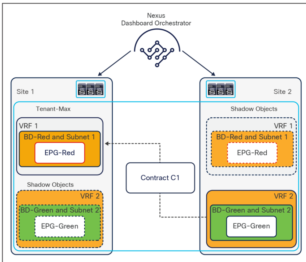
Figure 43. Layer 3 inter-VRF communication across sites
