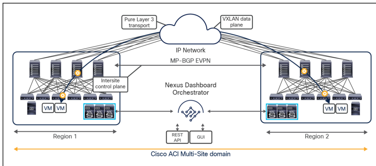
Figure 5. Cisco ACI Multi-Site architecture
