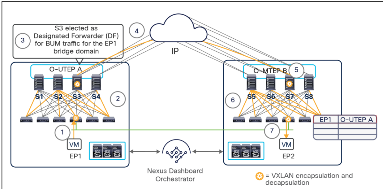
Figure 69. Layer 2 BUM traffic across sites
