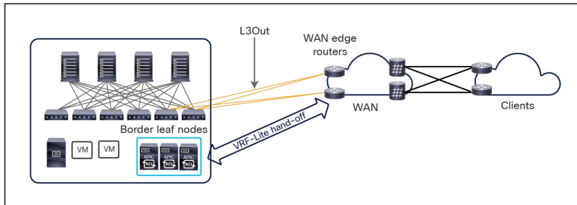
Figure 97. L3Out connections on border leaf nodes
