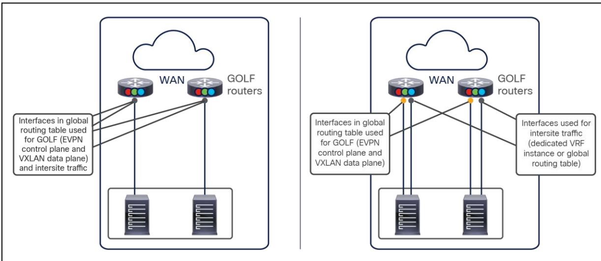
Figure 135. Shared or dedicated physical connections for GOLF and Multi-Site deployments
