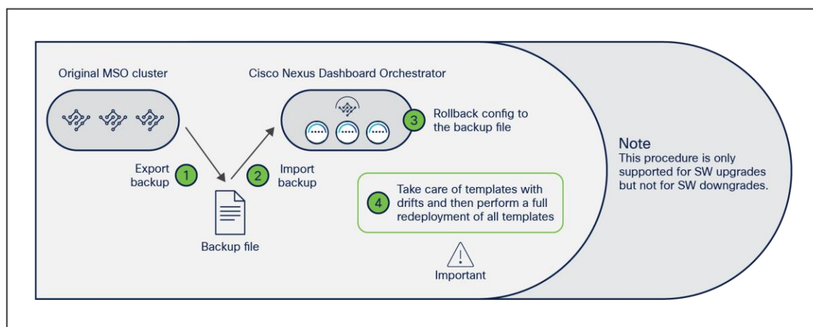
Figure 26. Upgrading and/or migrating procedure between MSO and NDO
