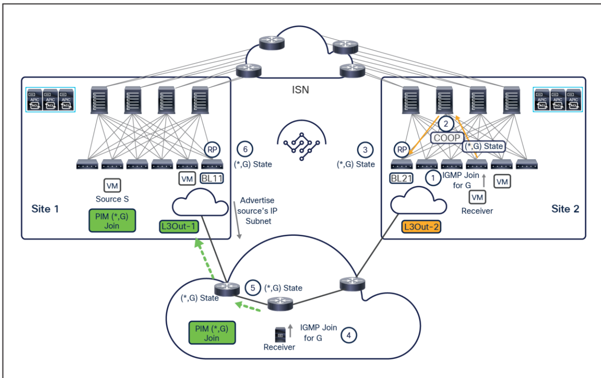
Figure 81. Control plane activity when internal and external receivers join multicast group G
