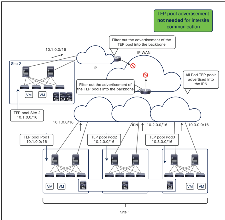
Figure 96. TEP pool advertisement out of each pod and filtering it out in the backbone
