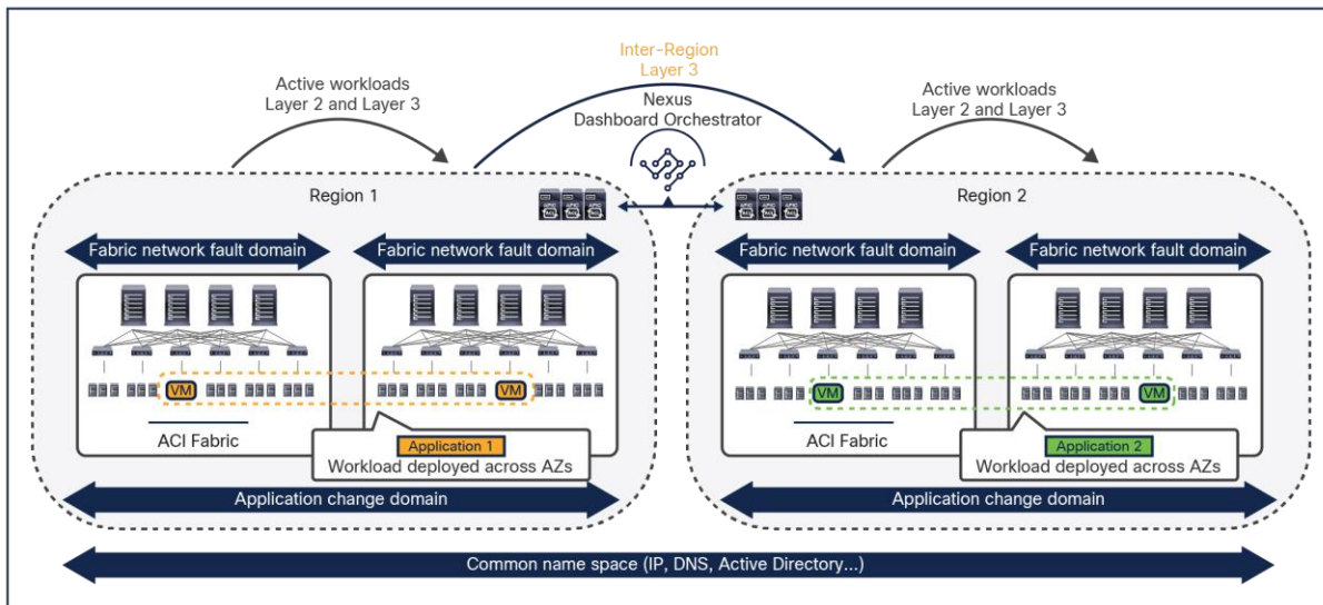
Figure 3. Change and network fault domains isolation
