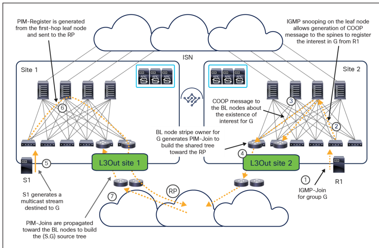
Figure 128. Control-plane interactions for a PIM-ASM use case
