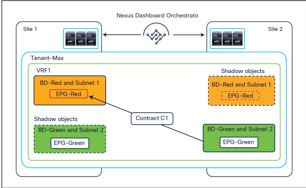
Figure 41. Layer 3 intra-VRF Layer 3 communication across sites
