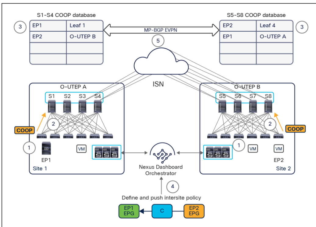
Figure 66. Cisco ACI Multi-Site overlay control plane
