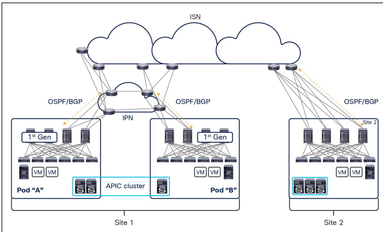
Figure 91. Separate network infrastructures for IPN and ISN connectivity
