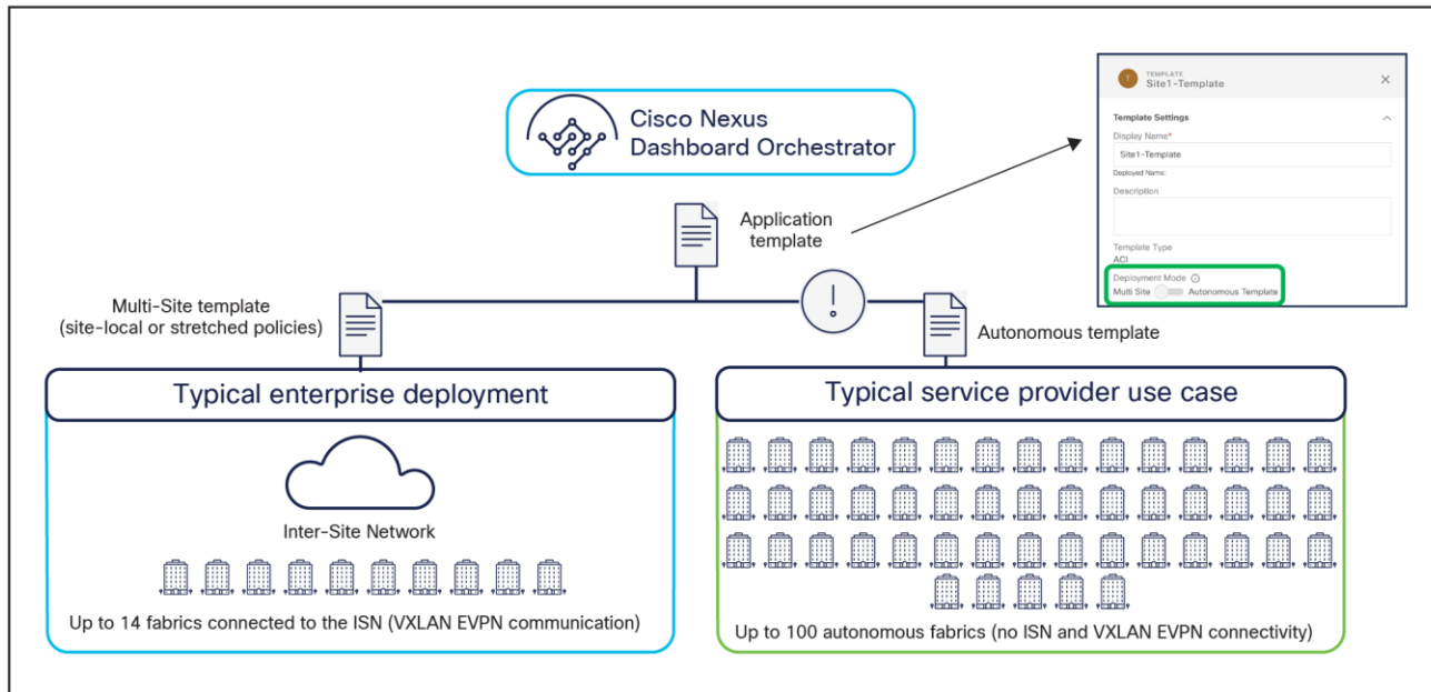
Figure 31. Multi-Site and autonomous application templates
