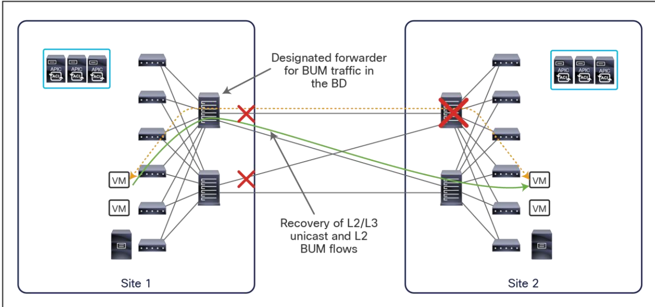
Figure 65. Traffic recovery in remote spine's failure scenario with full-mesh connections
