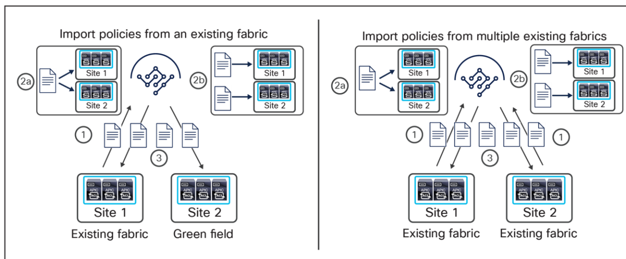
Figure 124. Importing policies into Cisco Nexus Dashboard Orchestrator
