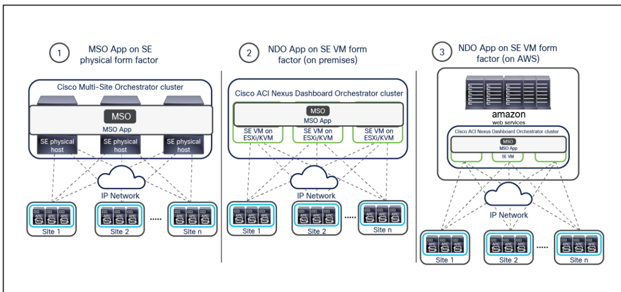
Figure 132. MSO cluster deployment on different Cisco Application Services Engine form factors
