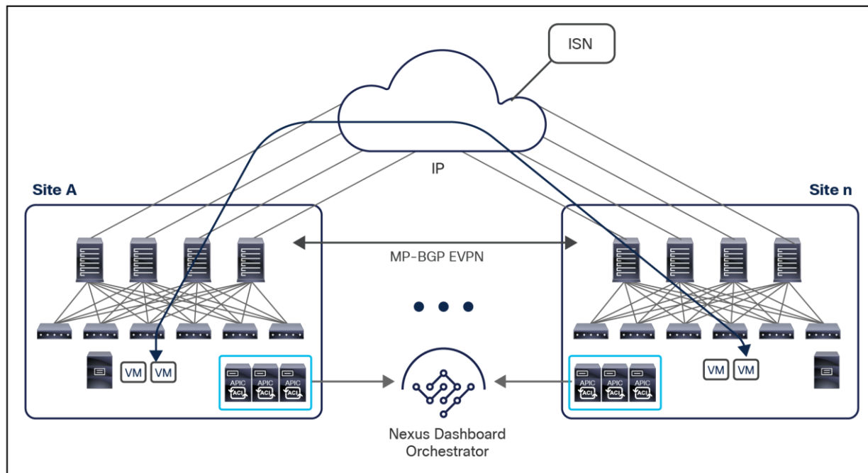
Figure 56. Intersite Network (ISN)
