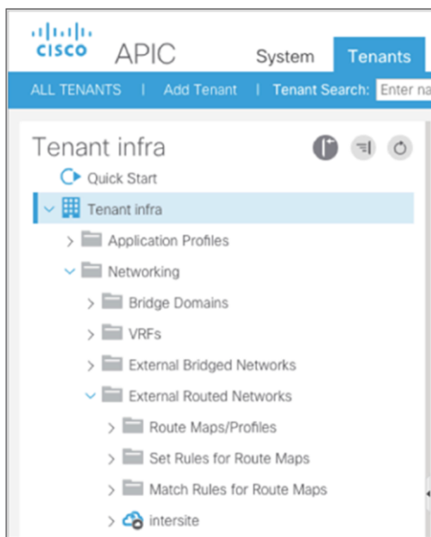
Figure 126. Creation of Intersite L3Out in Cisco APIC
