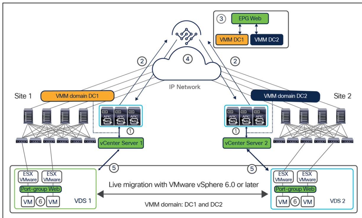
Figure 121. Live migration across VMM domains with VMware vCenter 6.0 or later
