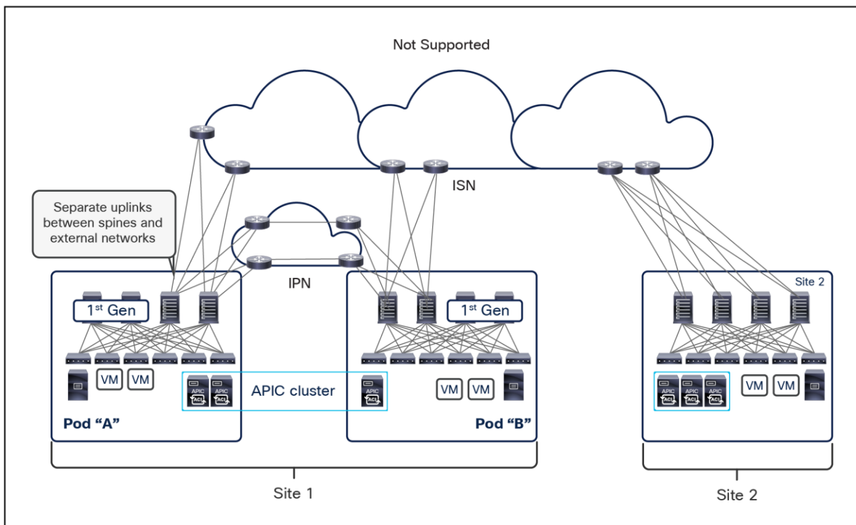
Figure 92. Use of separate uplinks between spines and external networks
