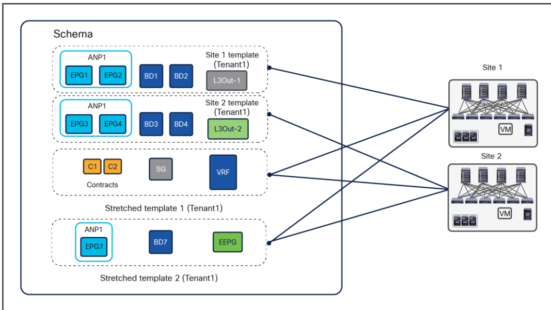
Figure 30. Best practices to define application templates inside a schema, beginning with NDO 4.x releases
