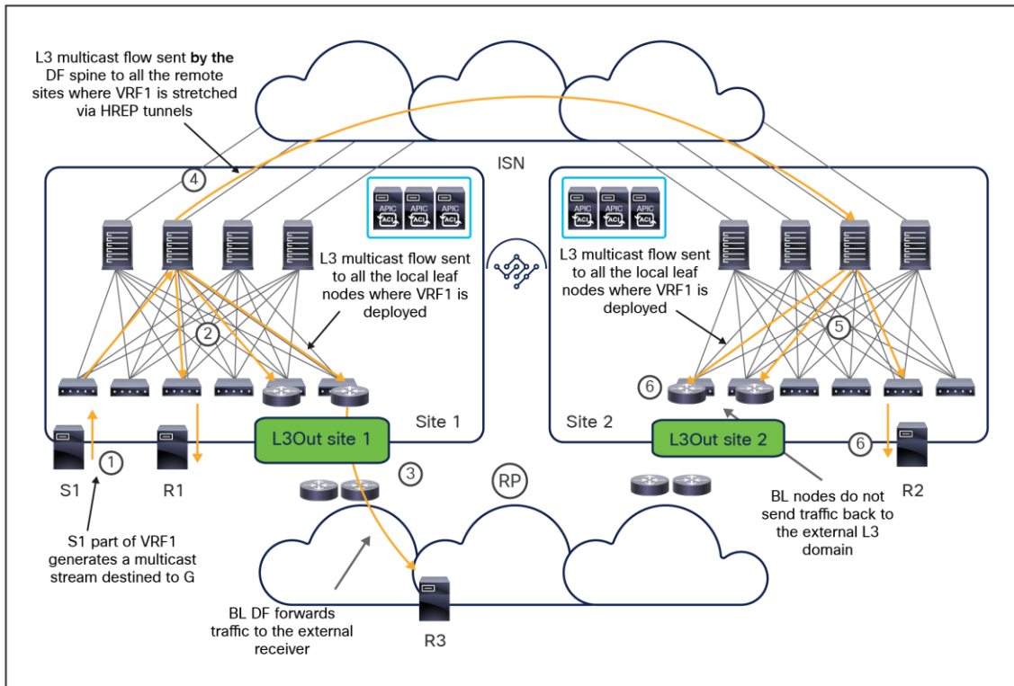
Figure 129. Layer 3 multicast forwarding between internal source and internal/external receivers
