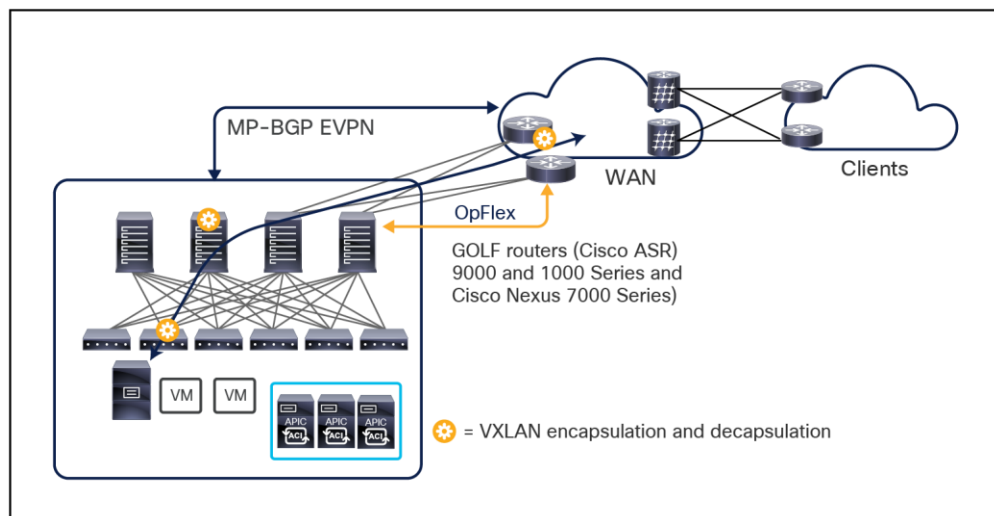
Figure 99. GOLF L3Out connections
