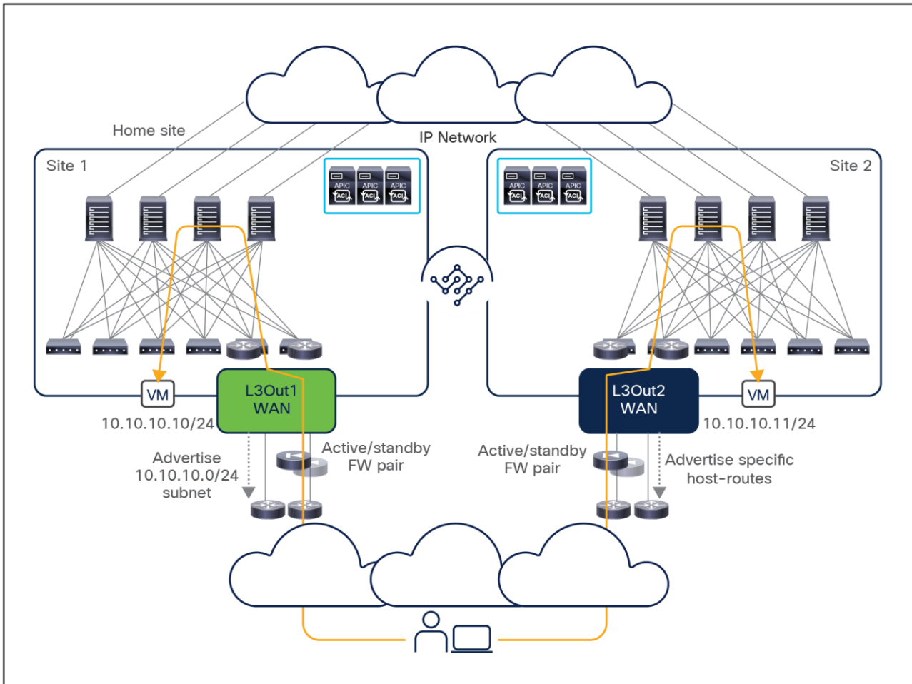
Figure 107. Home site deployment
