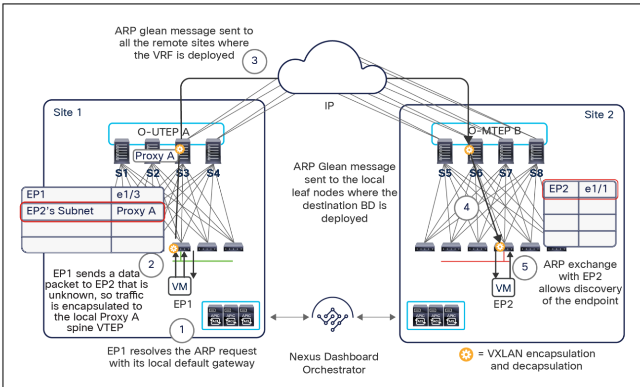
Figure 75. ARP Glean functionality for an inter-subnet communication use case
