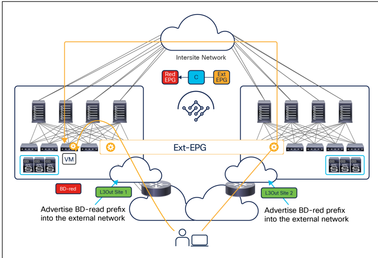
Figure 118. Creation of suboptimal inbound traffic path
