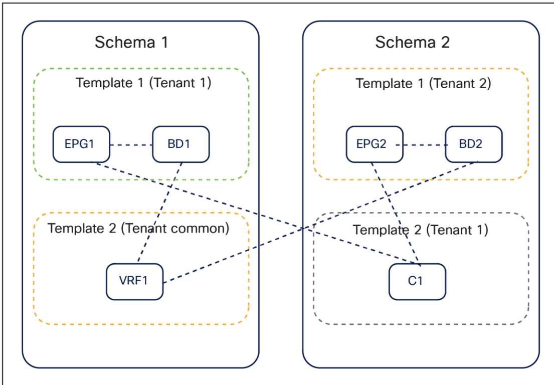
Figure 28. Referencing objects across application templates and across schemas
