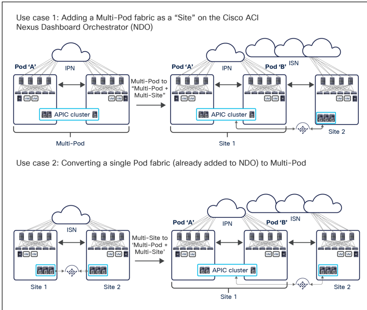
Figure 89. Use cases for integrating Cisco ACI Multi-Pod and Cisco ACI Multi-Site
