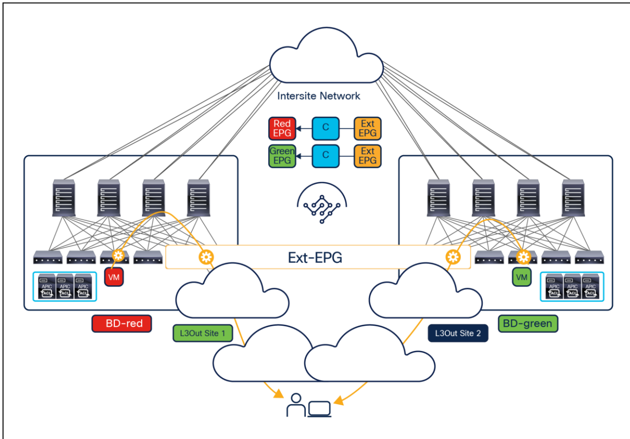
Figure 114. Optimal outbound traffic path
