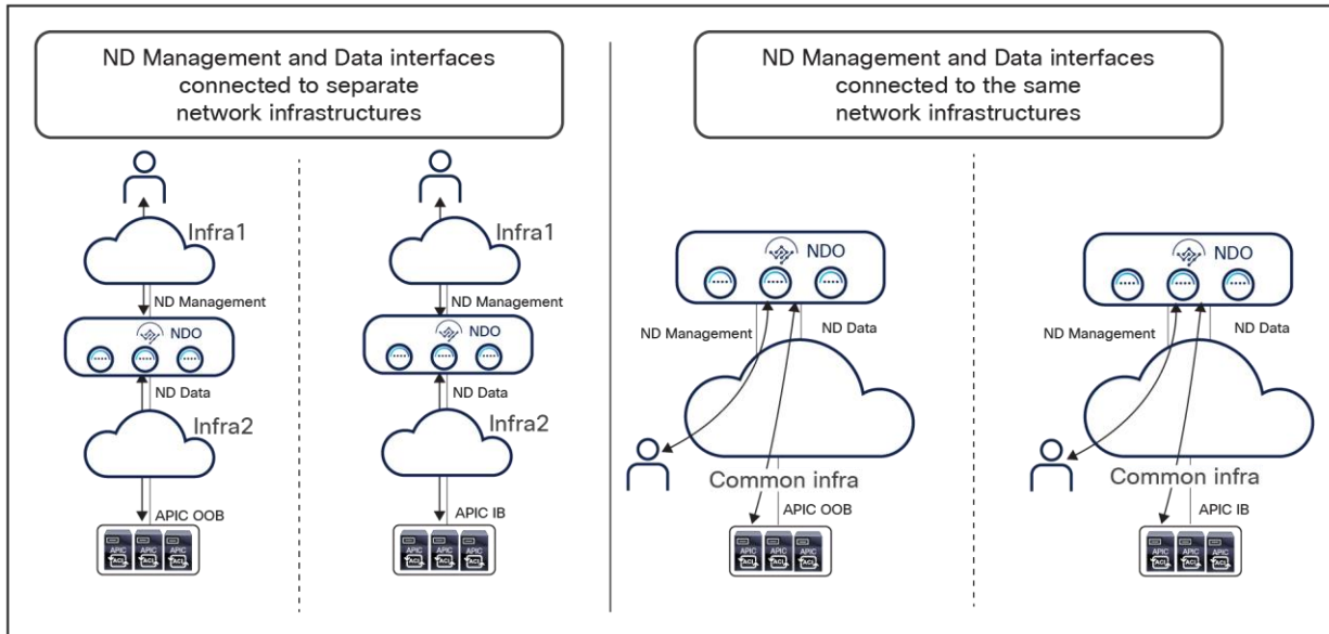
Figure 22. Nexus Dashboard compute node interfaces
