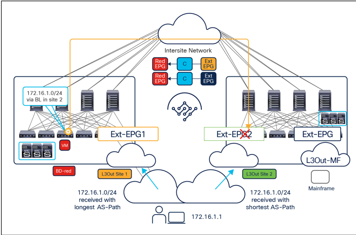
Figure 116. Possible dropping of outbound traffic when using separate external EPGs
