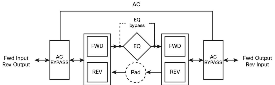
Figure 2. Block Diagram
