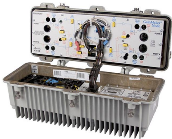
Figure 1. Cisco GainMaker 1 GHz High Output 4-Port Node with 85/105 MHz Split
