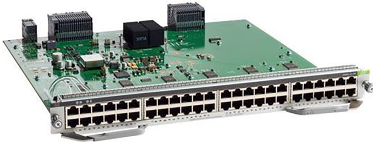
Figure 10. Cisco Catalyst 9400 Series 48-Port 10/100/1000 (RJ-45) Line Card (C9400-LC-48T)
