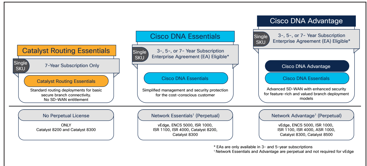
Figure 1. Cisco DNA SD-WAN and Routing software subscription offer structure
