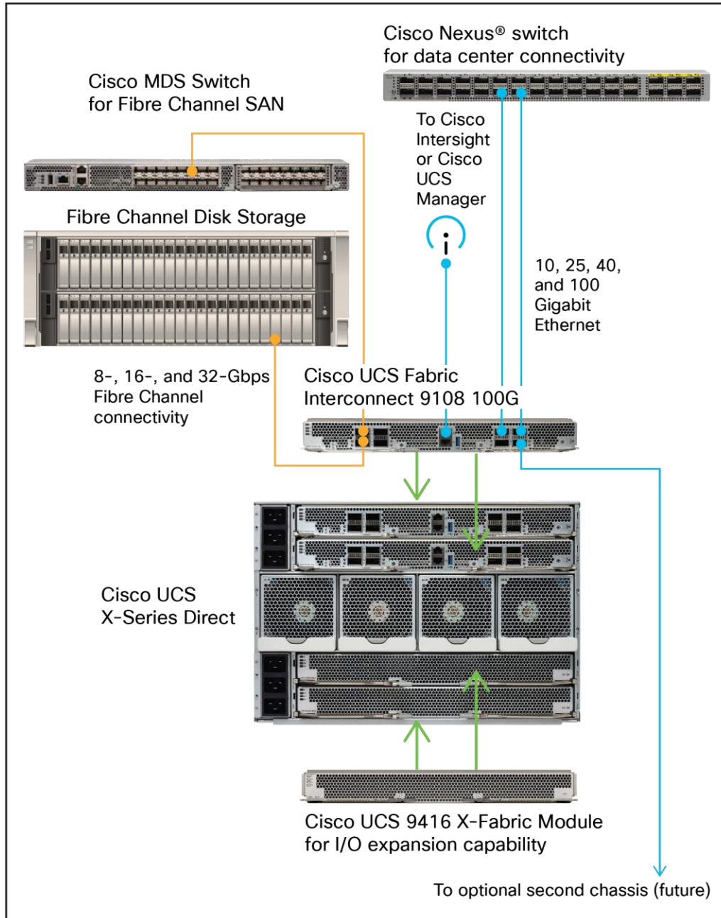
Figure 1. Cisco UCS X-Series Direct architectural options
