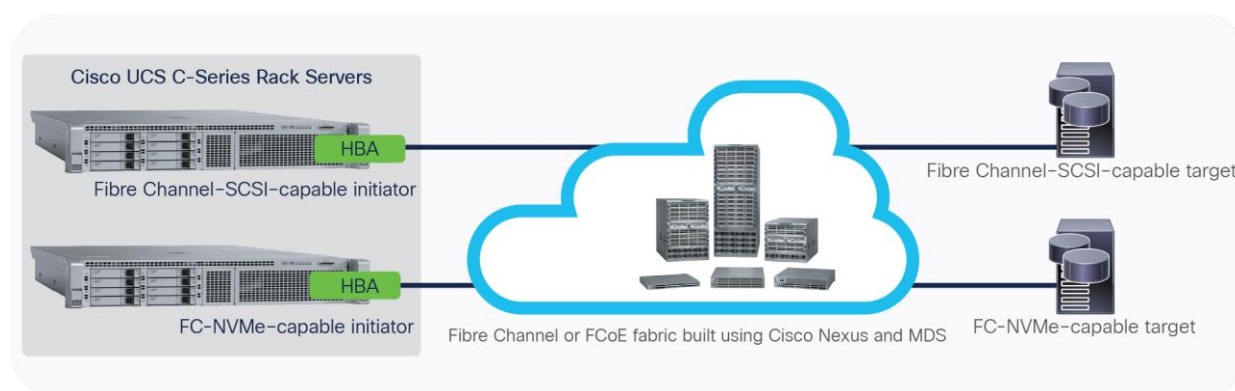
Figure 2. Seamless migration to FC-NVMe using Cisco Nexus and MDS
