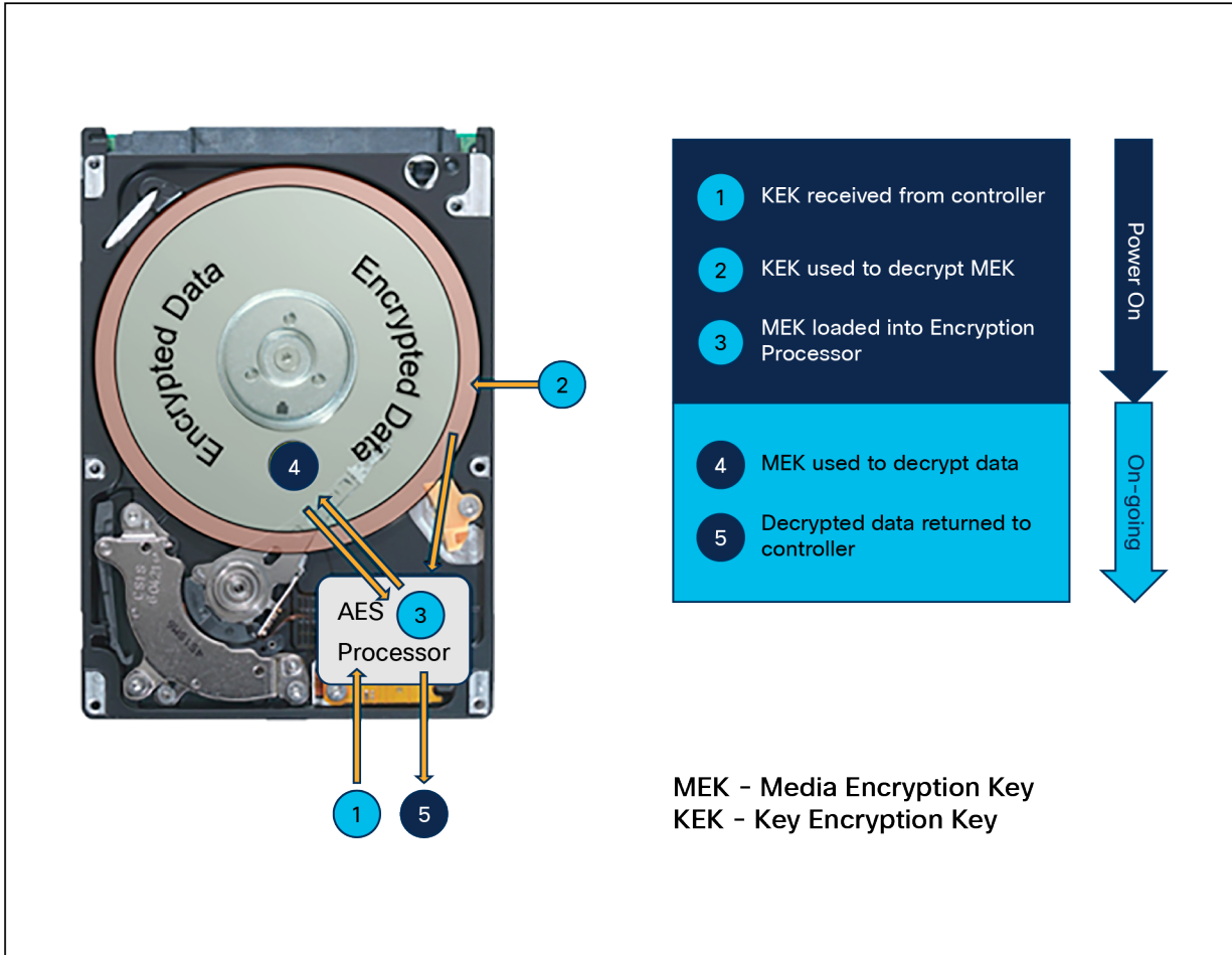
Figure 26. Anatomy of a self-encrypting drive
