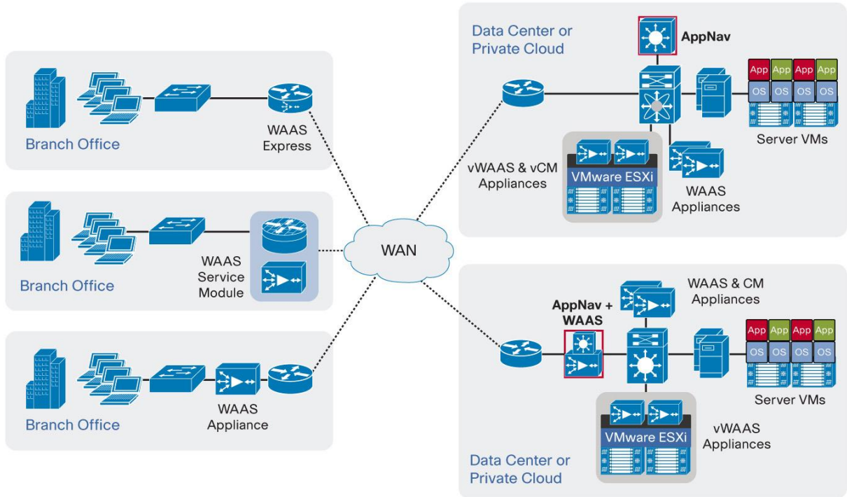
Figure 1. Cisco AppNav - WAAS Network Deployment Architecture
