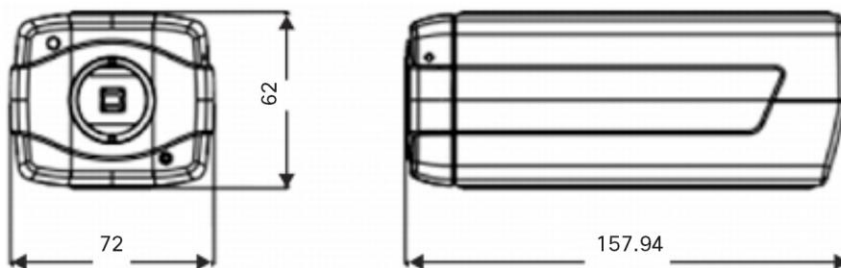
Figure 2. Cisco Video Surveillance 6500PD IP Camera Dimensions
