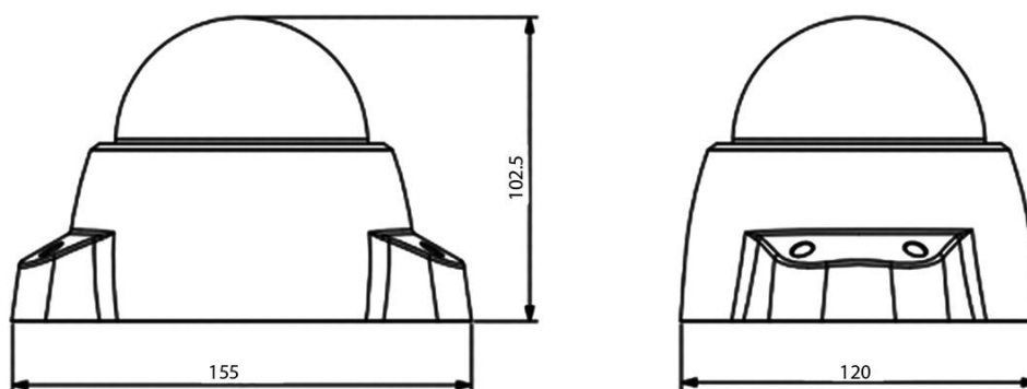
Figure 1. Cisco Video Surveillance 3421V IP Camera Dimensions
