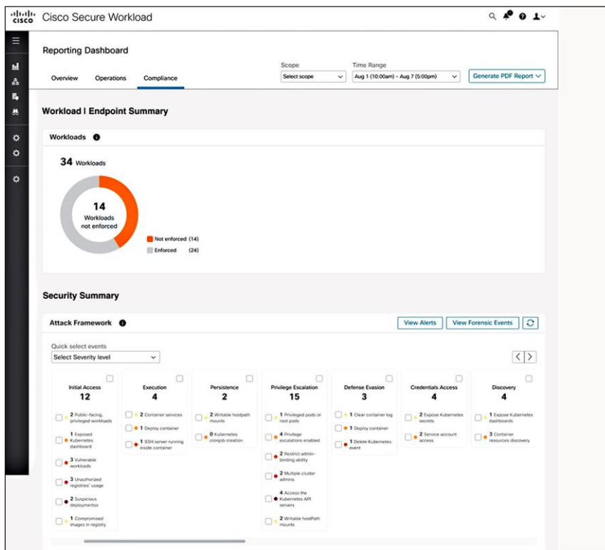
Figure 11. Reporting dashboard based on MITRE ATT&CK Framework
