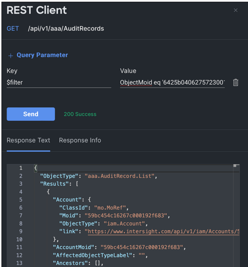
Figure 59. REST API query example using API explorer
