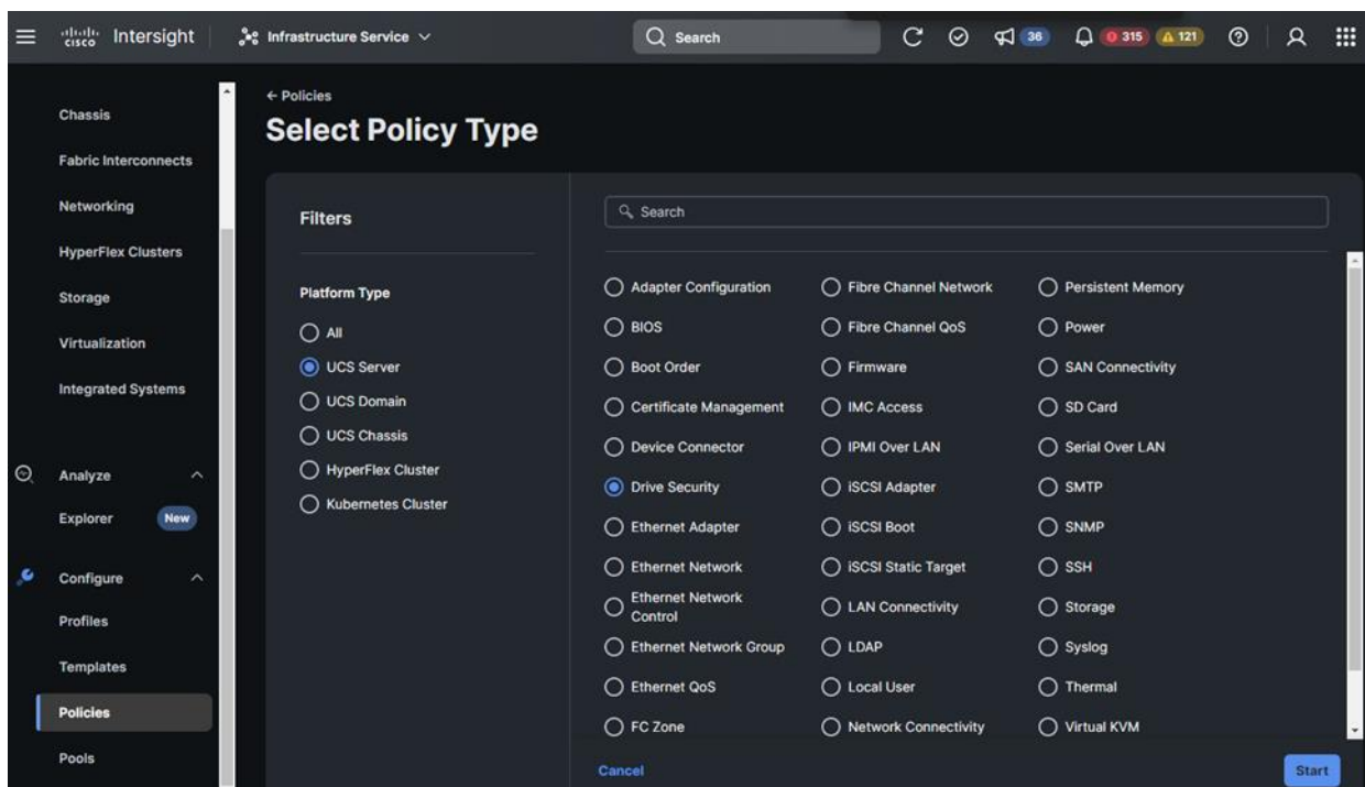
Figure 44. Drive-security policy
