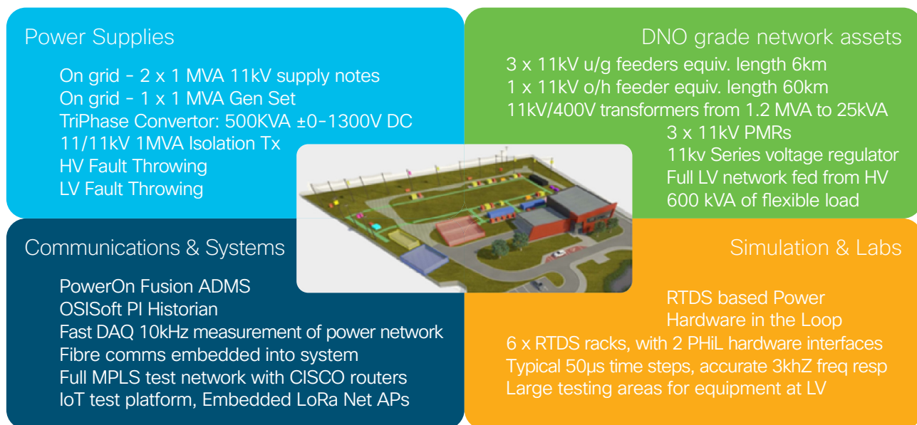
Figure 3 - High level architecture of the installed communication platform in PNDC
