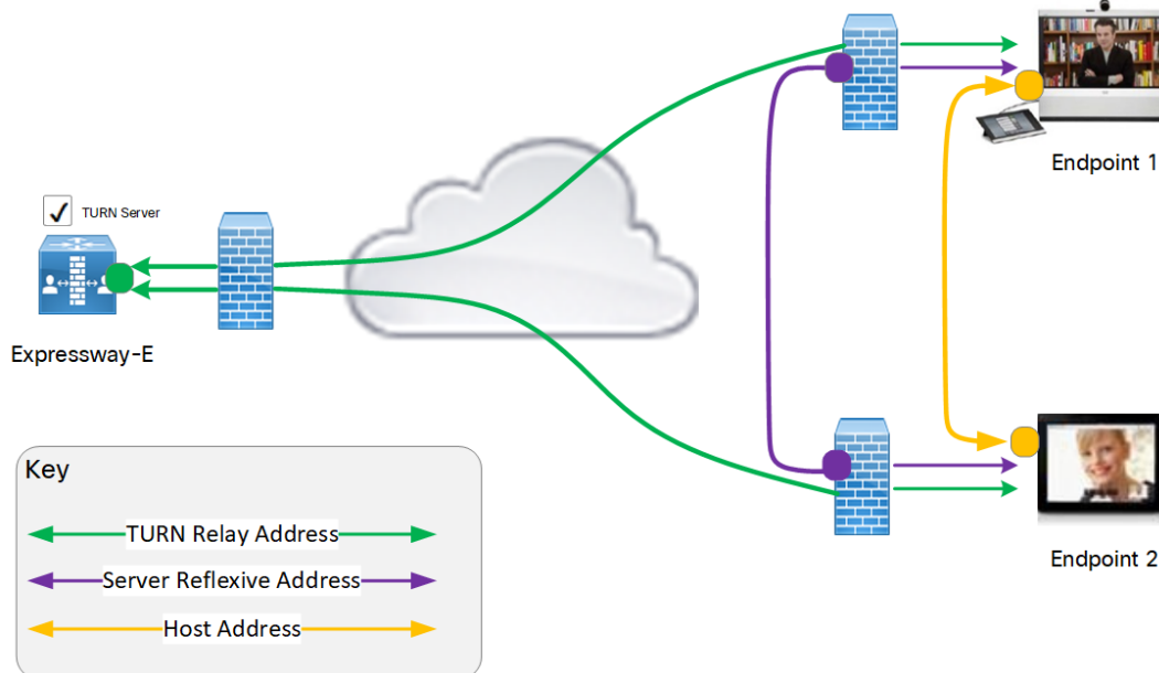
Figure 4 ICE Media connection paths
