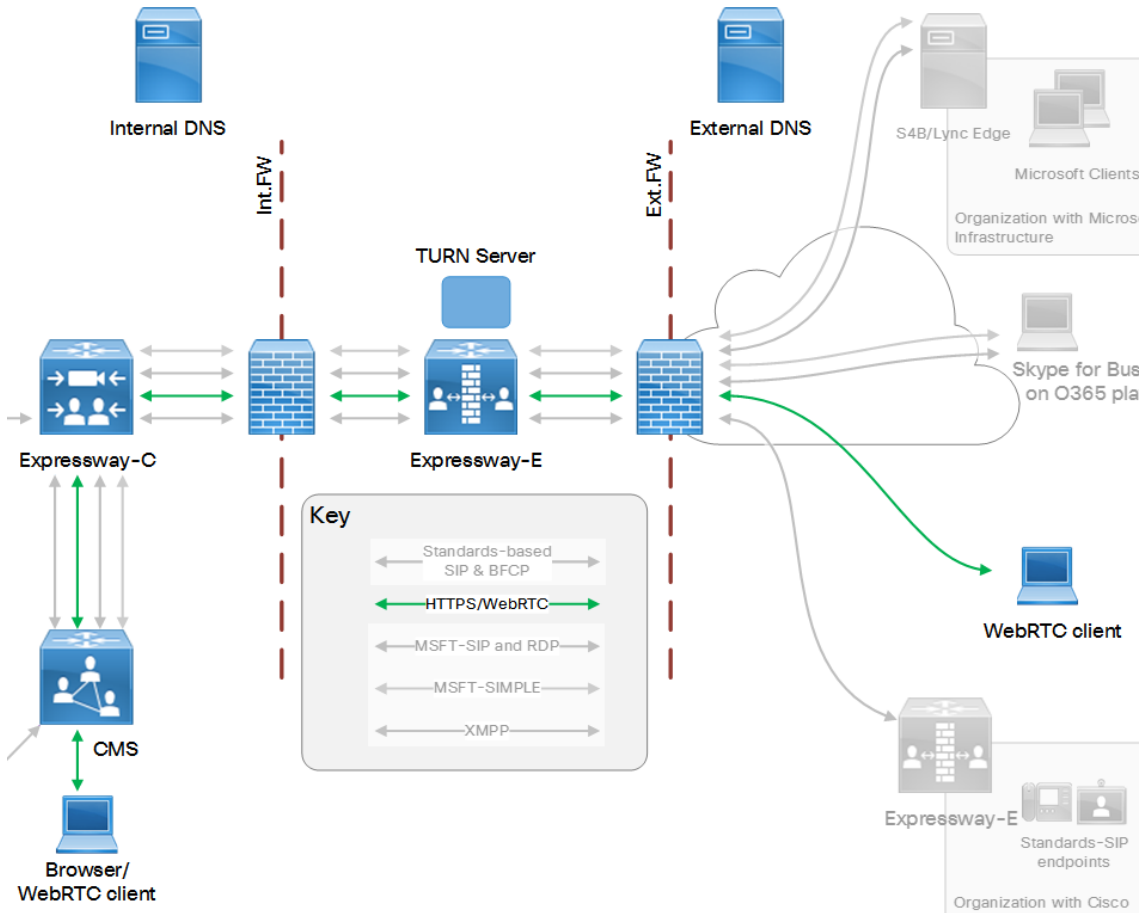
Figure 11 Meeting Server web proxy on Expressway
