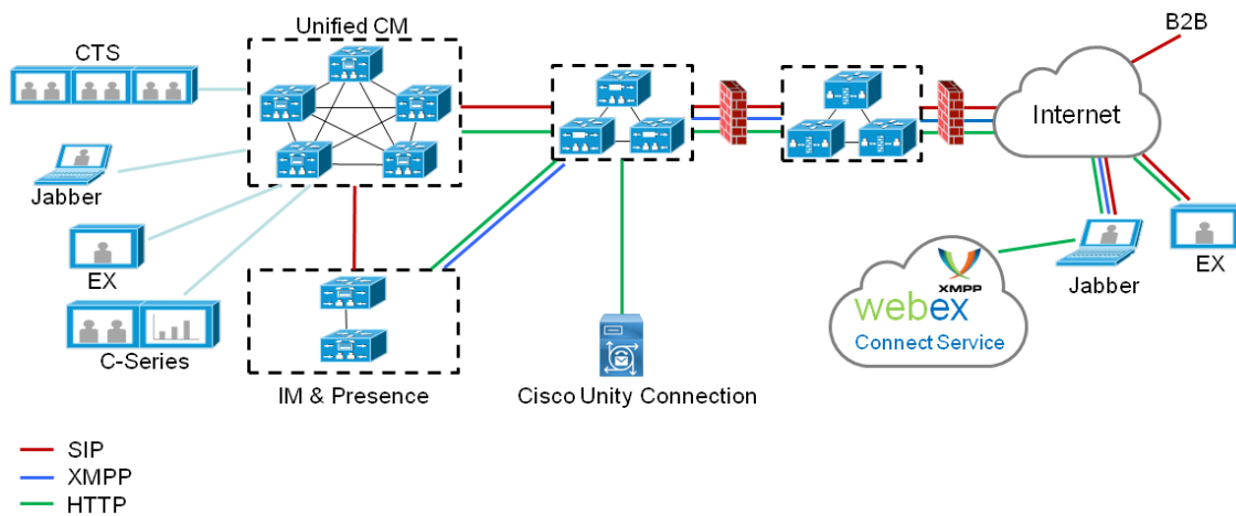
Figure 9 Unified Communications: Mobile and Remote Access
