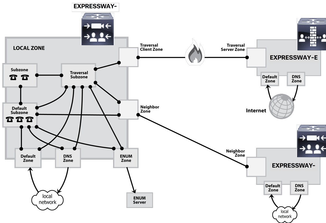
Figure 14 Example network diagram
