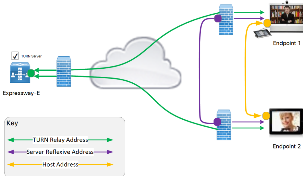
Figure 6 ICE Media connection paths
