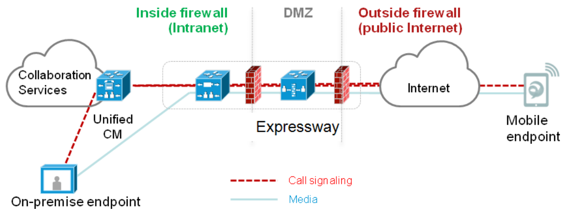
Figure 10 Typical call flow - signaling and media paths
