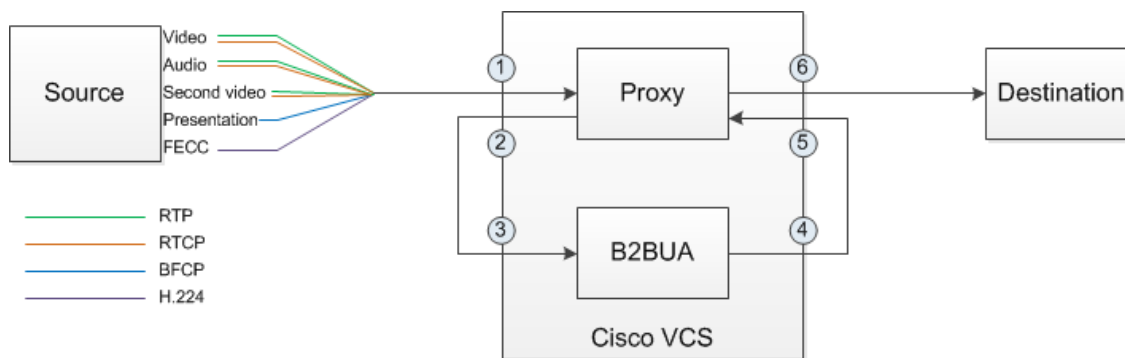
Figure 16 Maximum port allocation for a media traversal call
