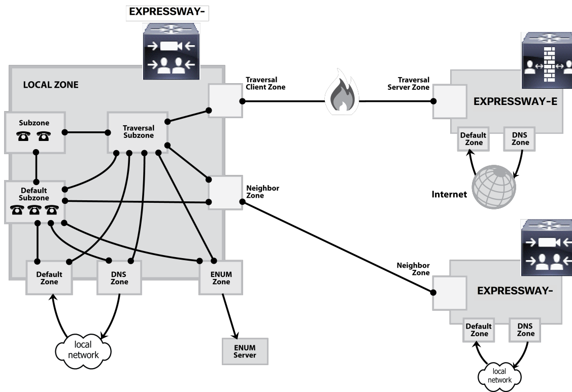
Figure 13 Example network diagram
