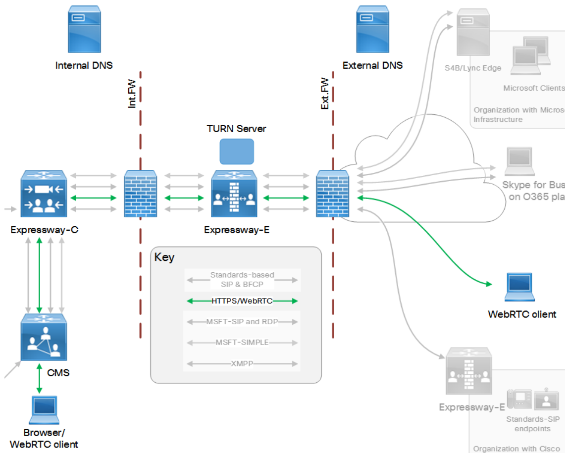
Figure 12 Meeting Server web proxy on Expressway
