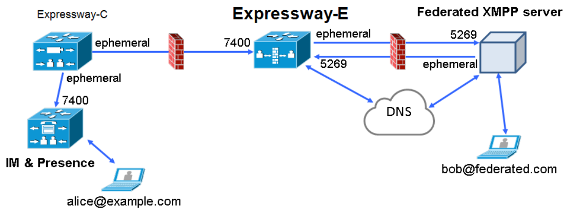
Figure 10 Message routing for XMPP federation
