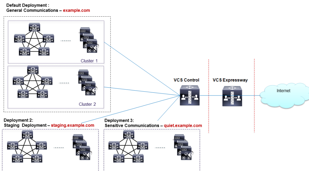
Figure 19 Multiple deployments to partition Unified Communications services accessed from outside the network
