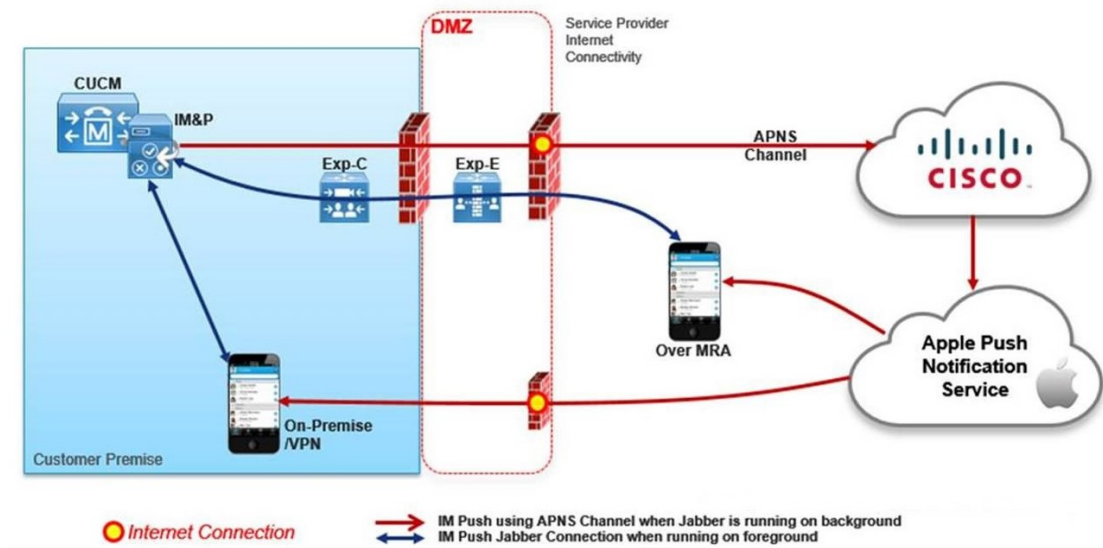
Figure 3 Example of Apple Push Notifications for CUCM IM&P and Jabber iOS
