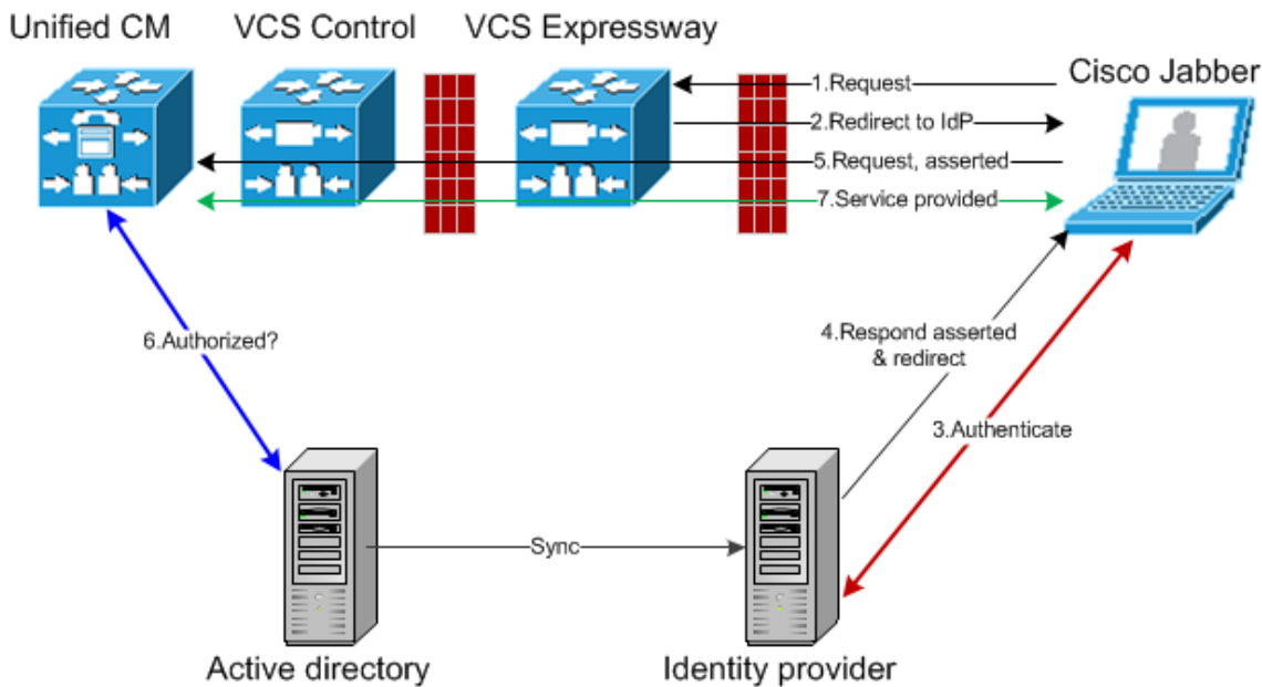
Figure 18 Remote single sign-on for on-premises UC services
