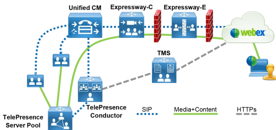
Figure 9. Architecture for Cisco CMR Hybrid
