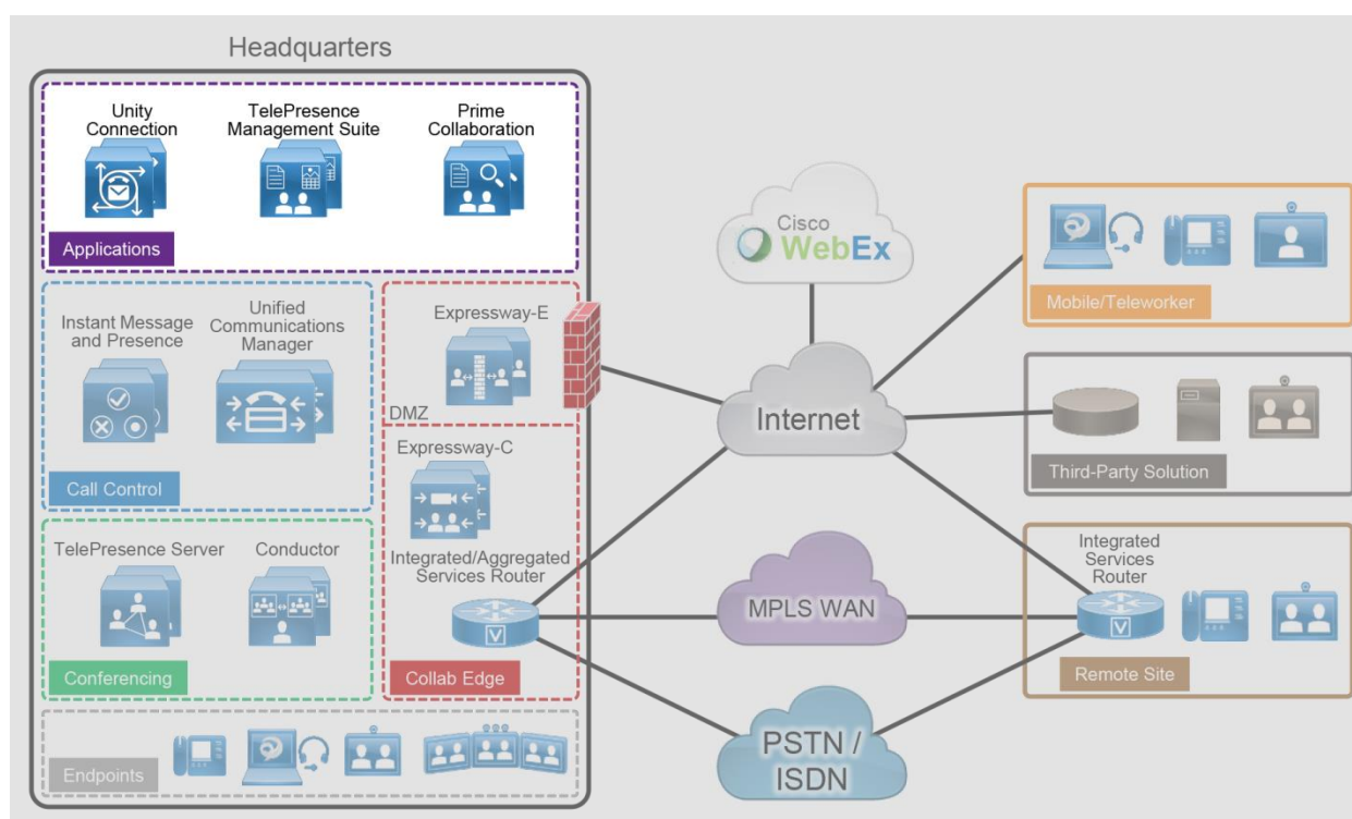
Figure 15. Architecture for Applications
