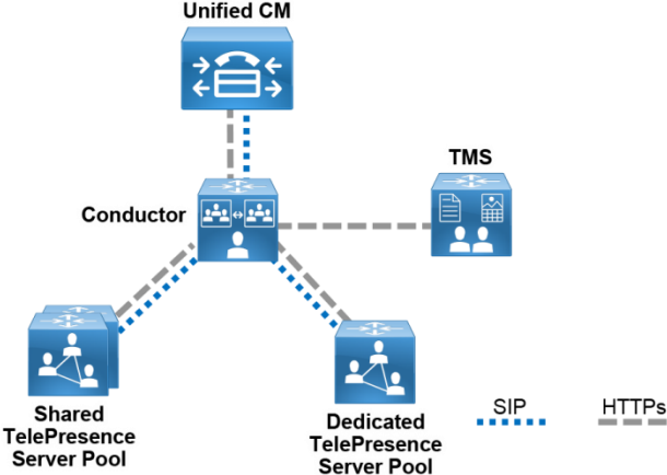
Figure 8. Architecture for Video Conferencing
