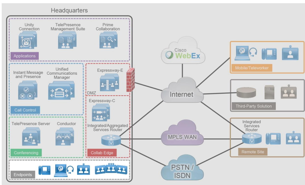
Figure 3. Architecture for Endpoints
