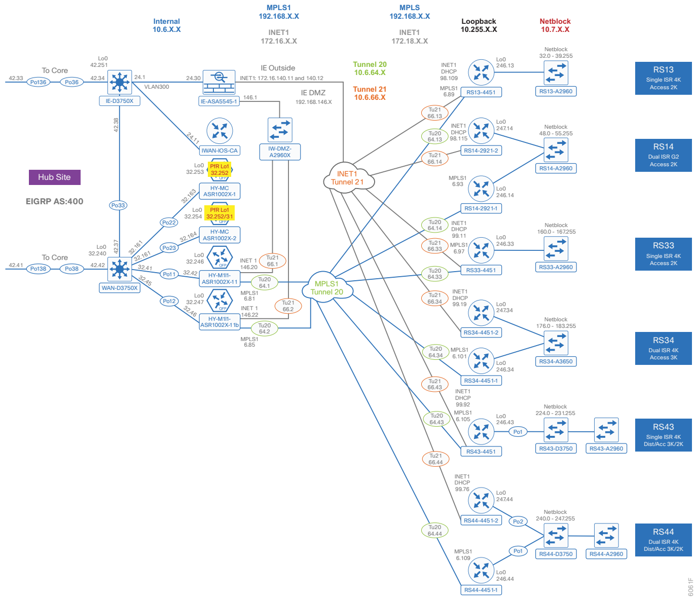
Figure 14 IWAN hybrid with MTT design model for EIGRP-Hub MC HA, hub BR scaling and IOS CA
