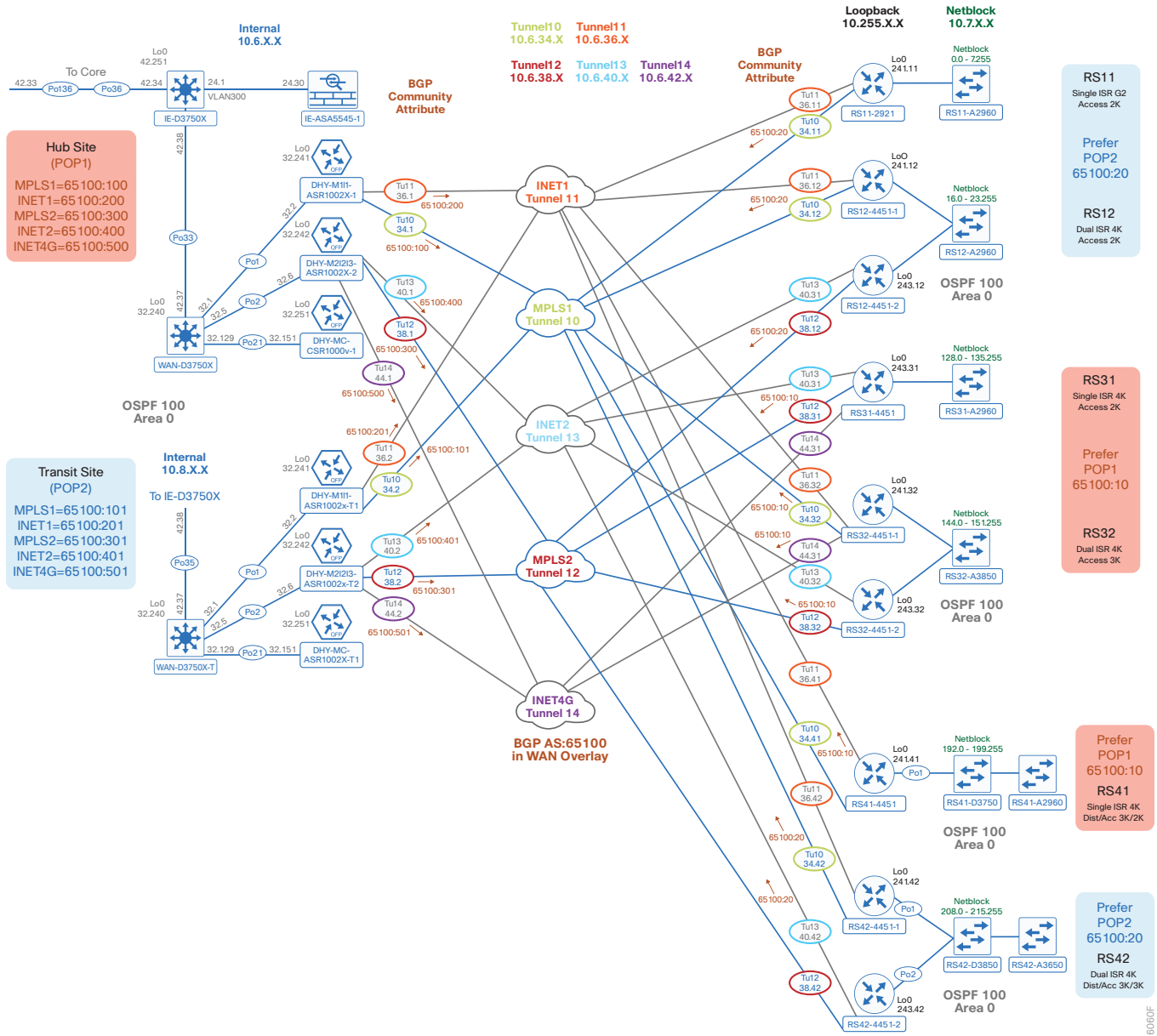
Figure 15 IWAN dual hybrid with PLR and MTT model for BGP and OSPF
