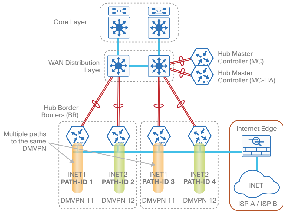
Figure 5 IWAN dual Internet model—Hub BR scalability
