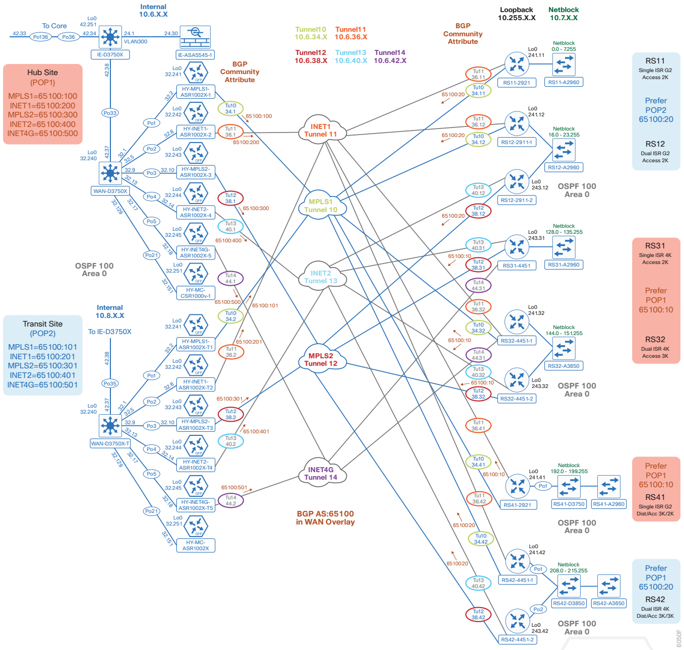
Figure 12 IWAN dual hybrid with PLR model for BGP and OSPF
