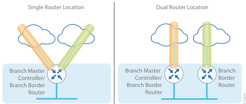
Figure 3 IWAN–Remote-site overview
