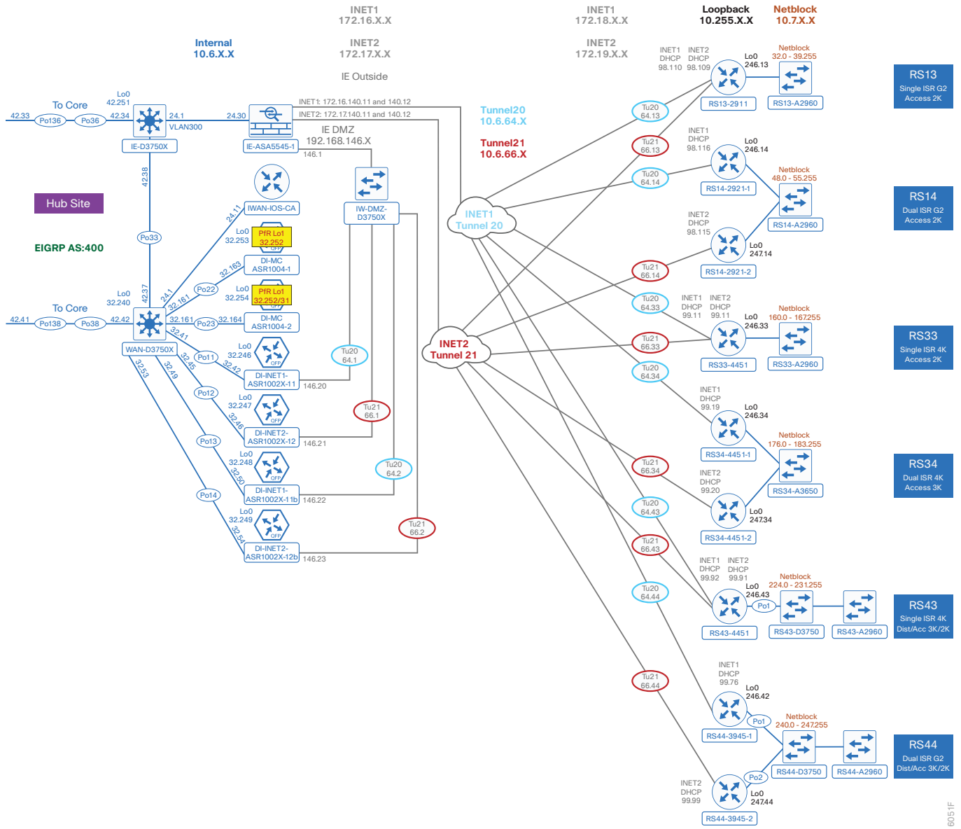
Figure 13 IWAN dual Internet model for EIGRP–Hub MC HA, hub BR scaling and IOS CA
