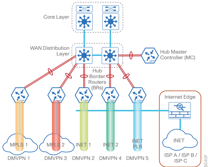
Figure 7 IWAN dual hybrid with PLR design model—WAN aggregation site overview
