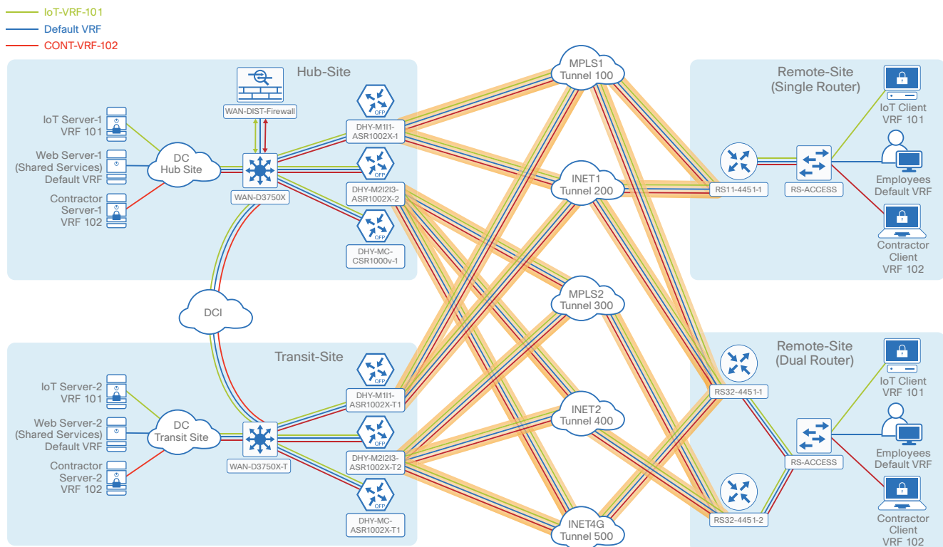
Figure 10 IWAN dual hybrid with PLR and Multi-VRF design model
