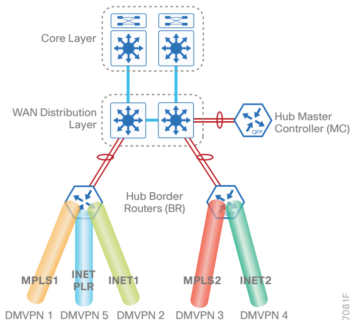
Figure 8 IWAN dual hybrid with PLR and MTT design model–WAN aggregation site overview
