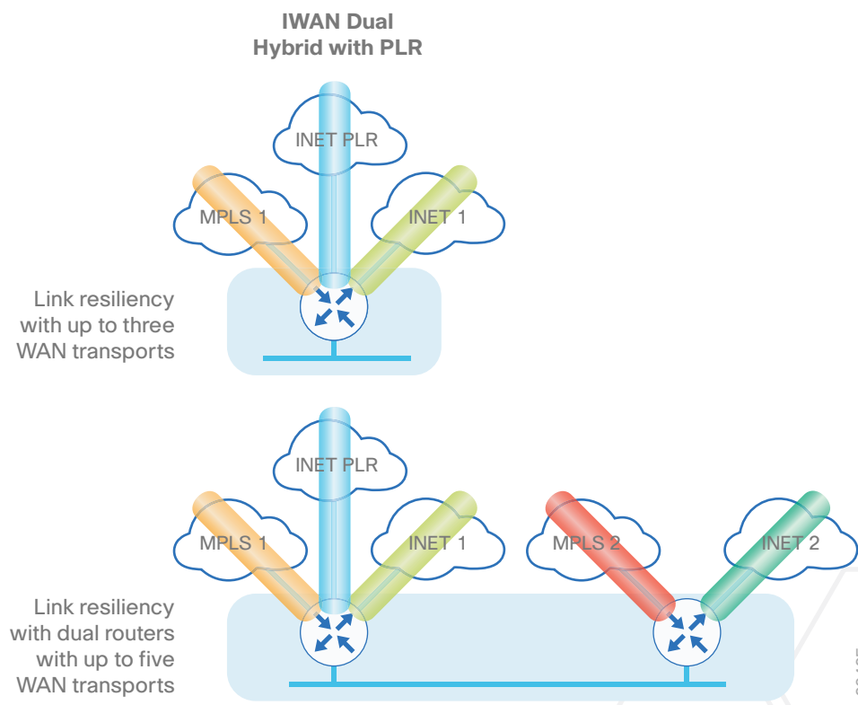
Figure 9 IWAN dual hybrid with PLR design model–Remote site options
