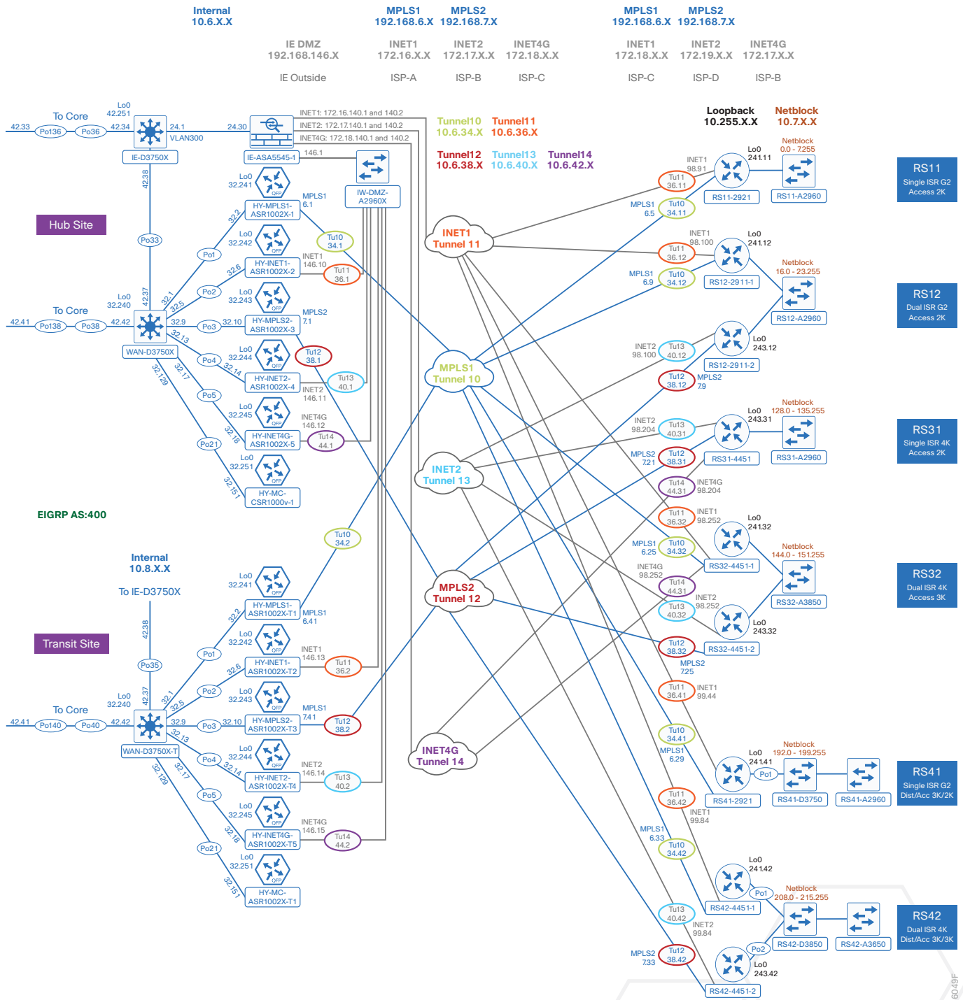
Figure 11 IWAN dual hybrid model w/ PLR model for EIGRP
