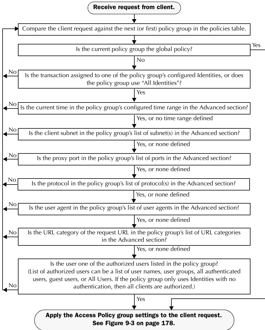
Figure 9-1 Policy Group Flow Diagram for Access Policies
