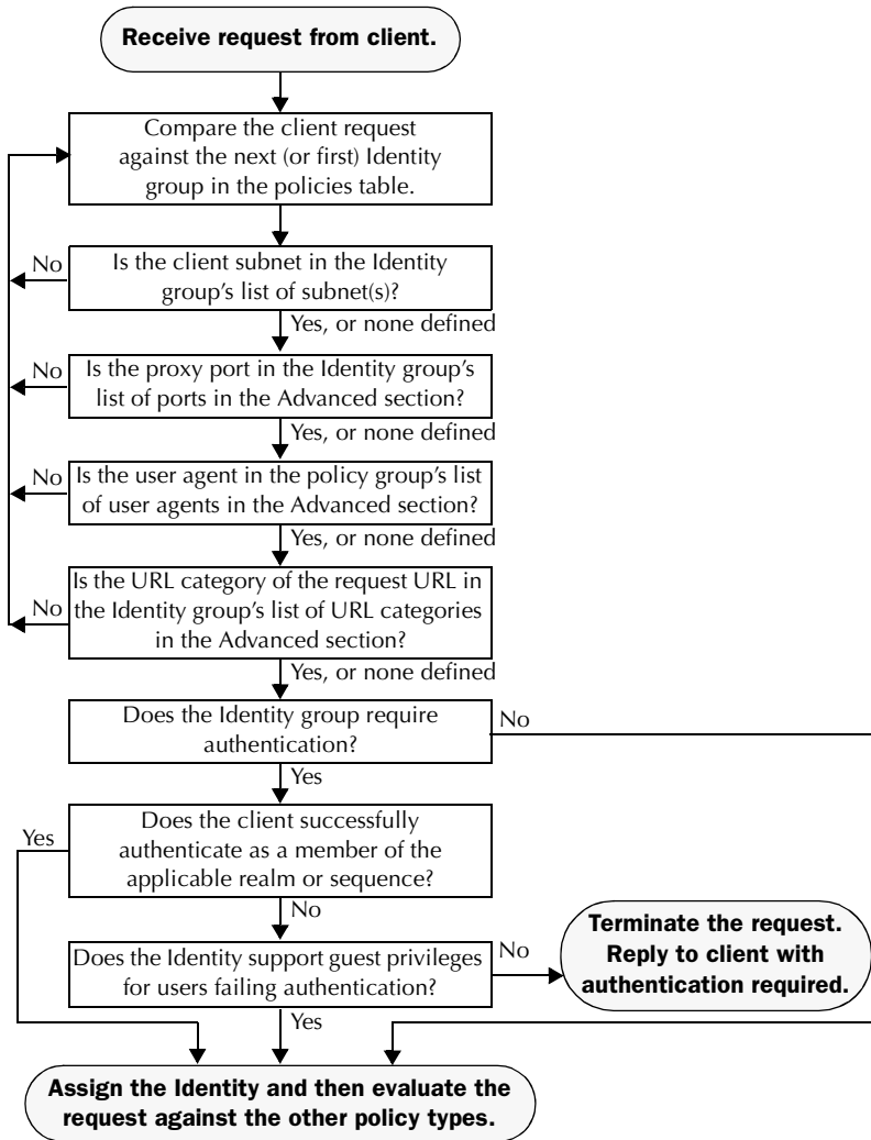
Figure 8-2 Policy Group Flow Diagram for Identities - No Surrogates and IP-Based Surrogates
