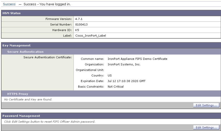
Figure 5-3 FIPS Management Console
