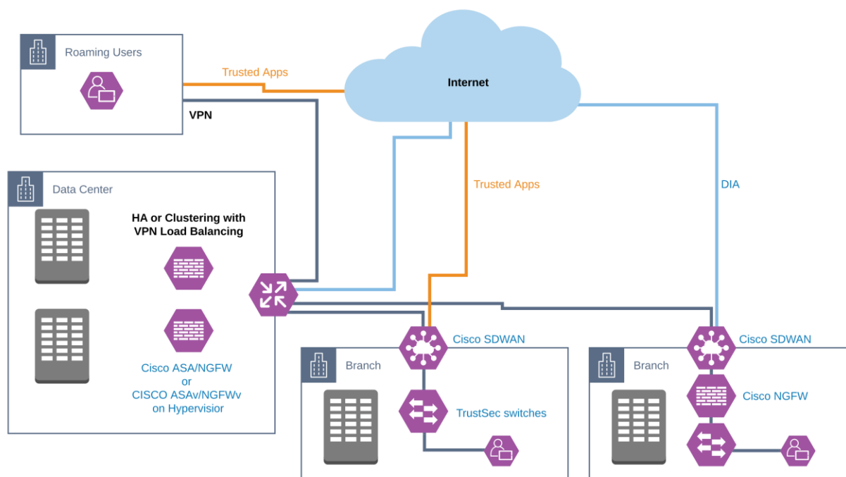
Figure 13. TIC 3.0 architecture
