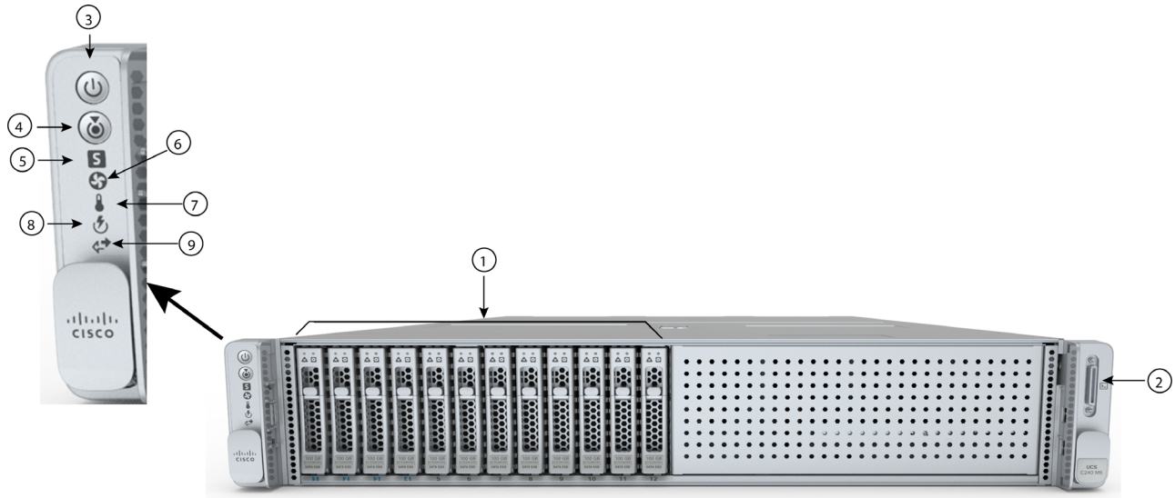
Figure 7 Chassis Front View (Option 3 - UCSC-C240-M6N)
