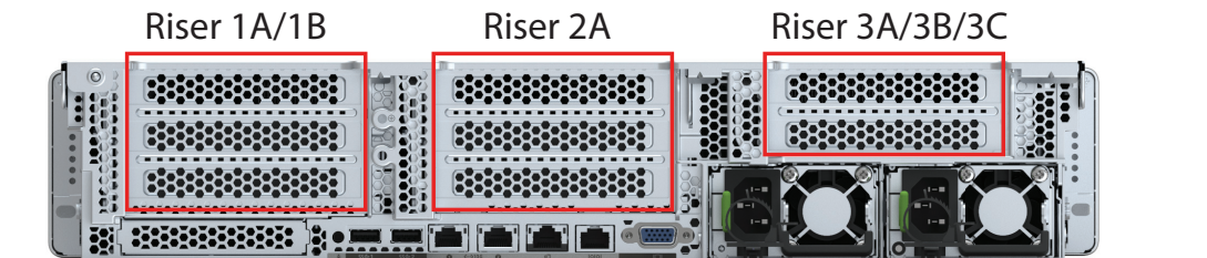
Figure 11 Riser Card Locations
