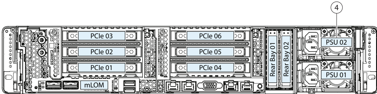
Figure 7 Riser Card 1 (slots 1, 2, and 3) and Riser Card 2 (slots 4, 5, and 6)
