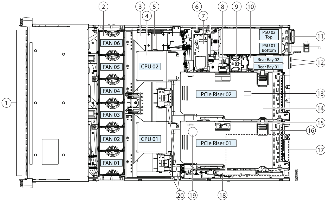
Figure 6 HX240c M5 LFF With Top Cover Off
