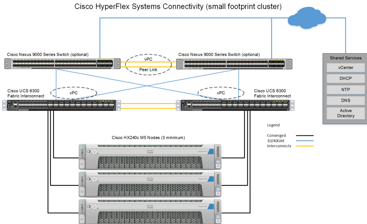
Figure 5 Small Footprint Cluster Using HX240c M5 LFF Nodes
