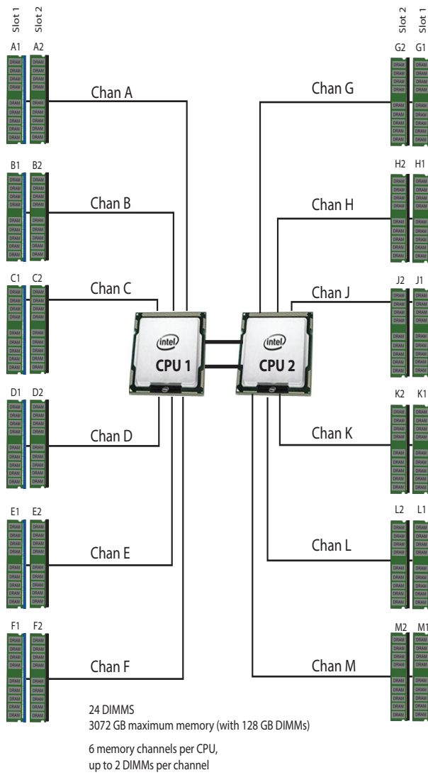
Figure 4 HX240 M5 LFF Memory Organization
