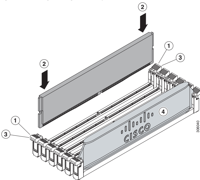
Figure 13 Replacing Memory
